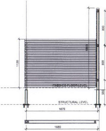
ELEVATION D
