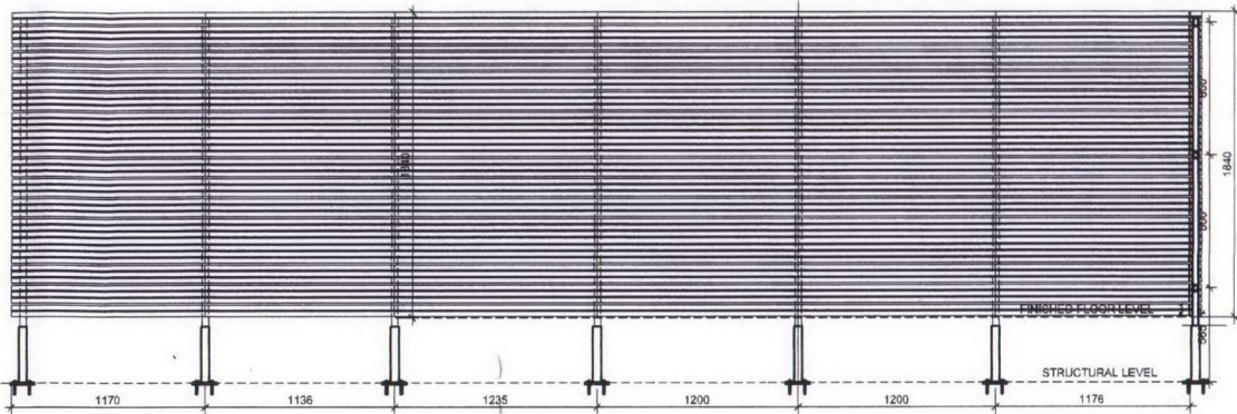
ELEVATION C
