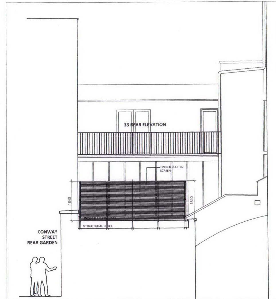
PROPOSED - No. 33 ELEVATION 1:100 (A3)
