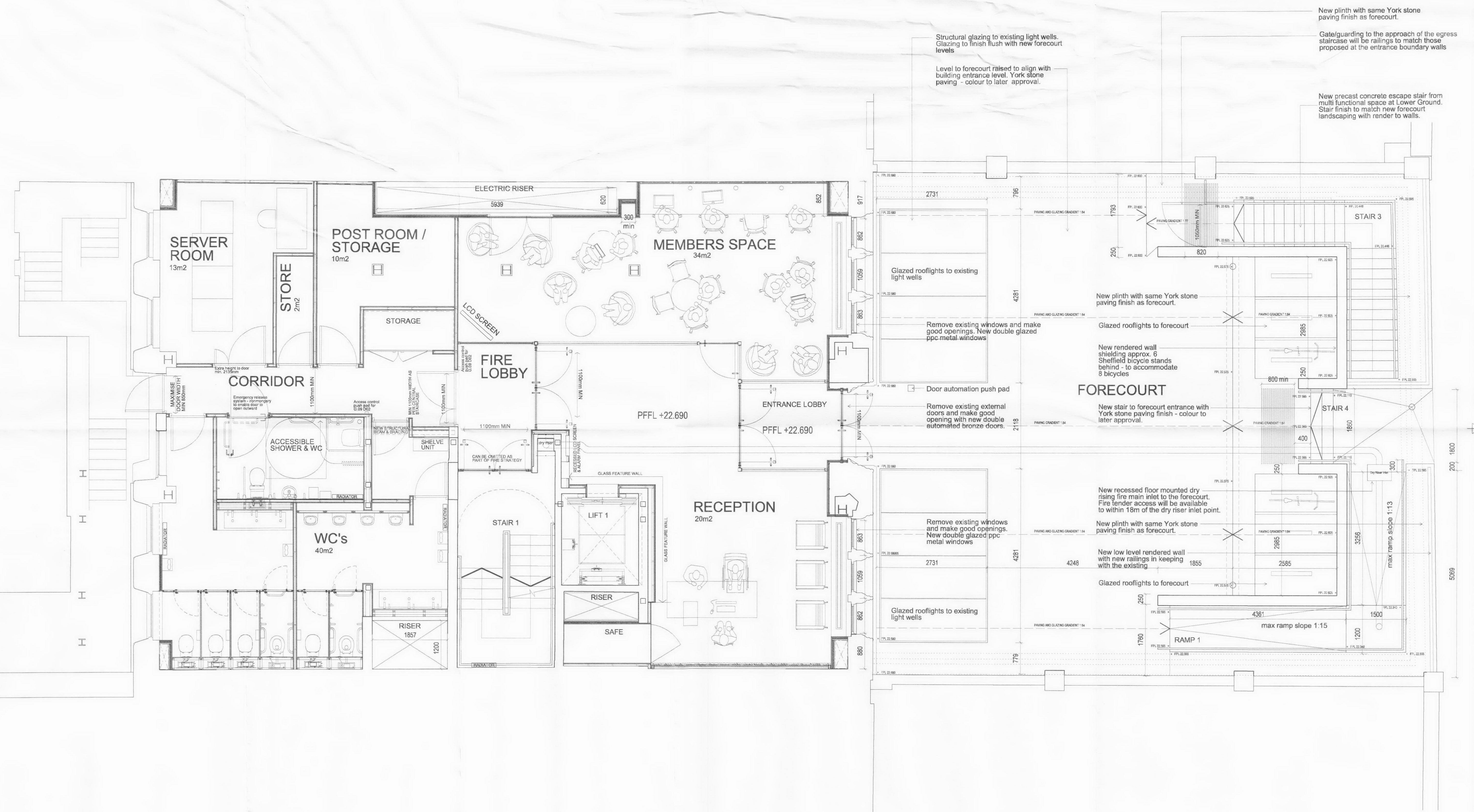
GROUND FLOOR PLAN - Existing Approved scheme
