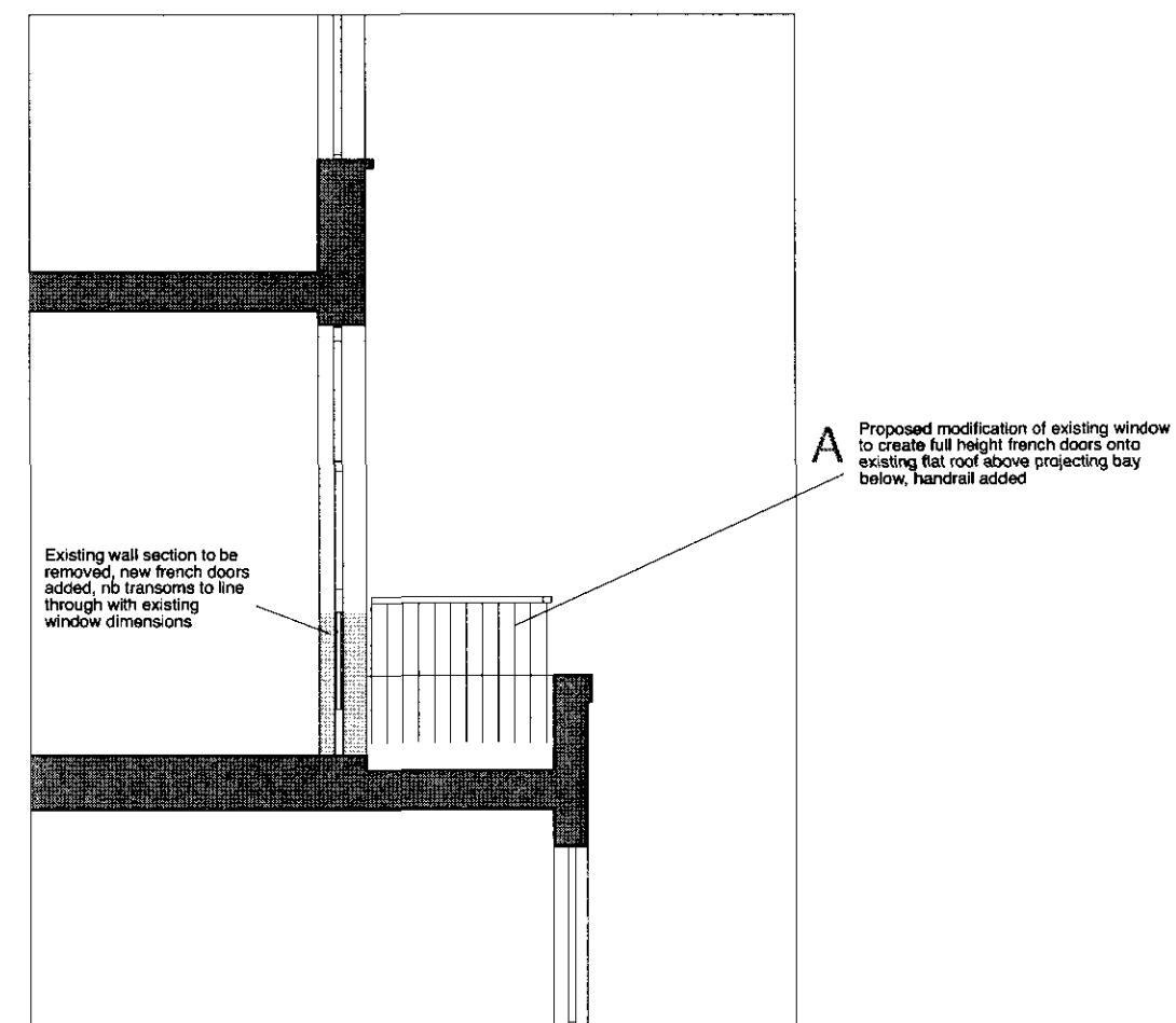
Section through rear second floor balcony and french doors
