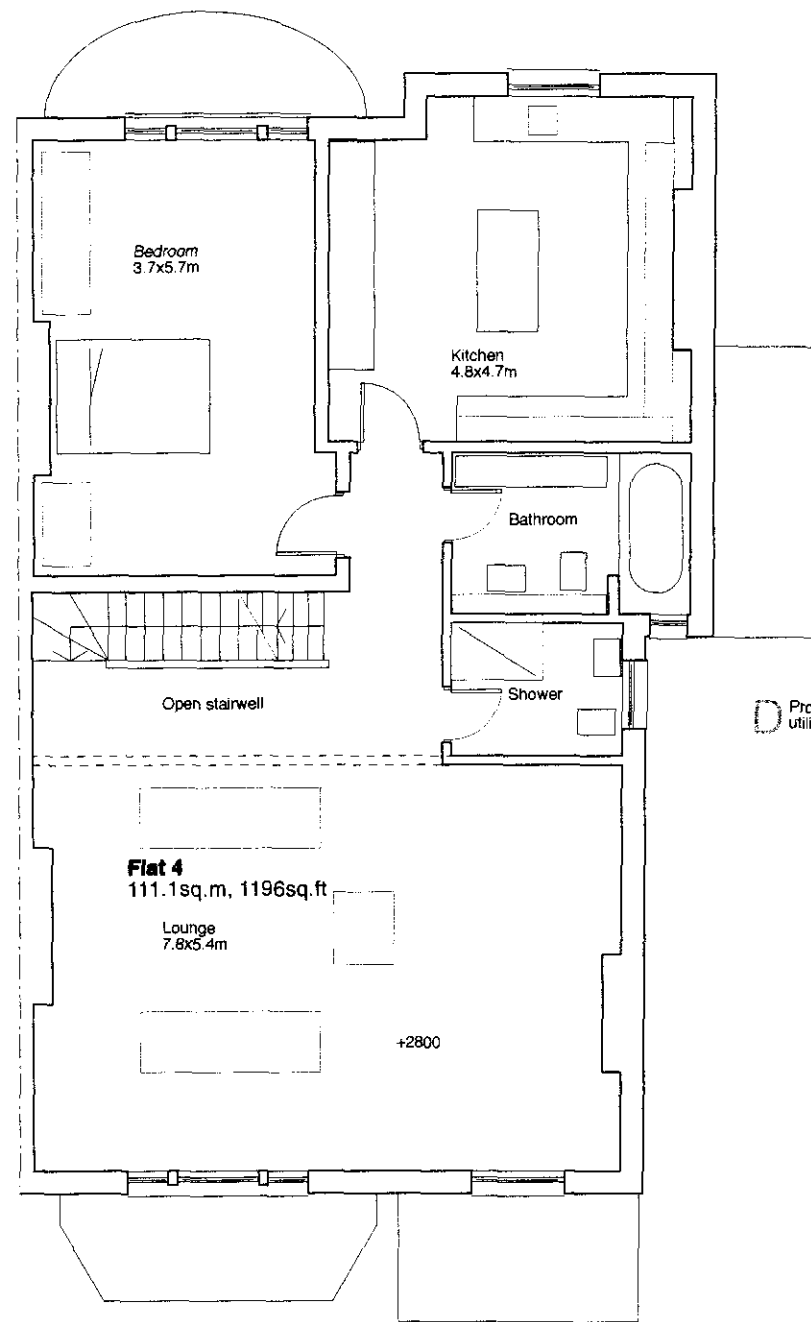
Second floor plan - as existing
