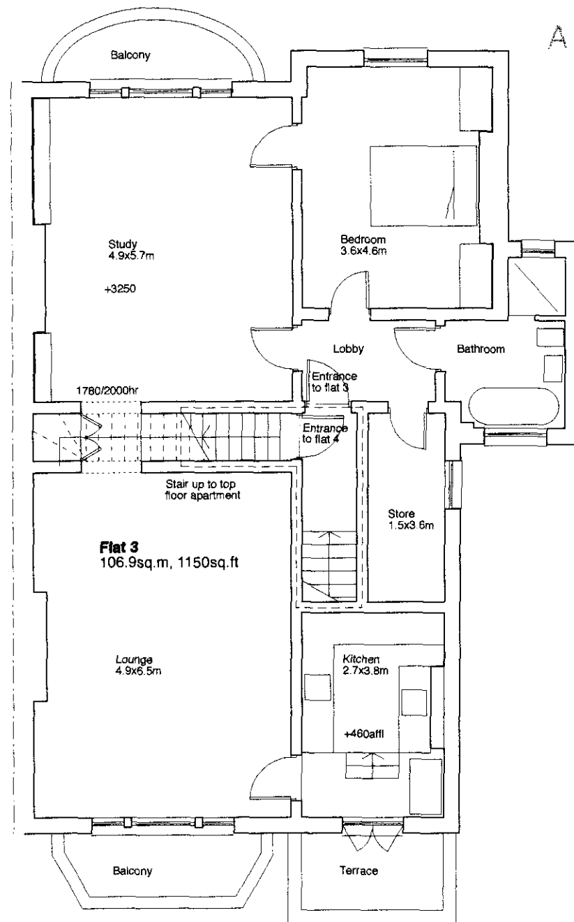
First floor plan - as existing
