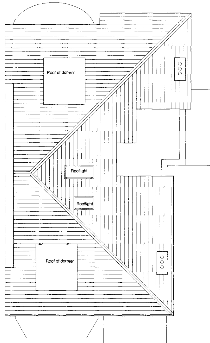
Roof plan - as existing
