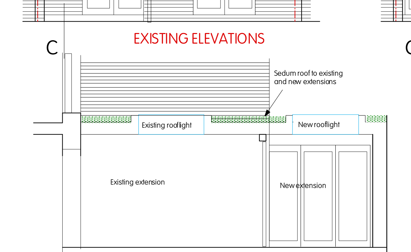
C SECTION
