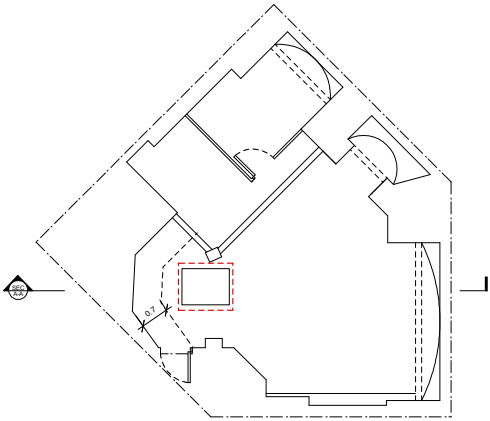
Basement Plan: Proposed Scale: 1:200 @ A3
