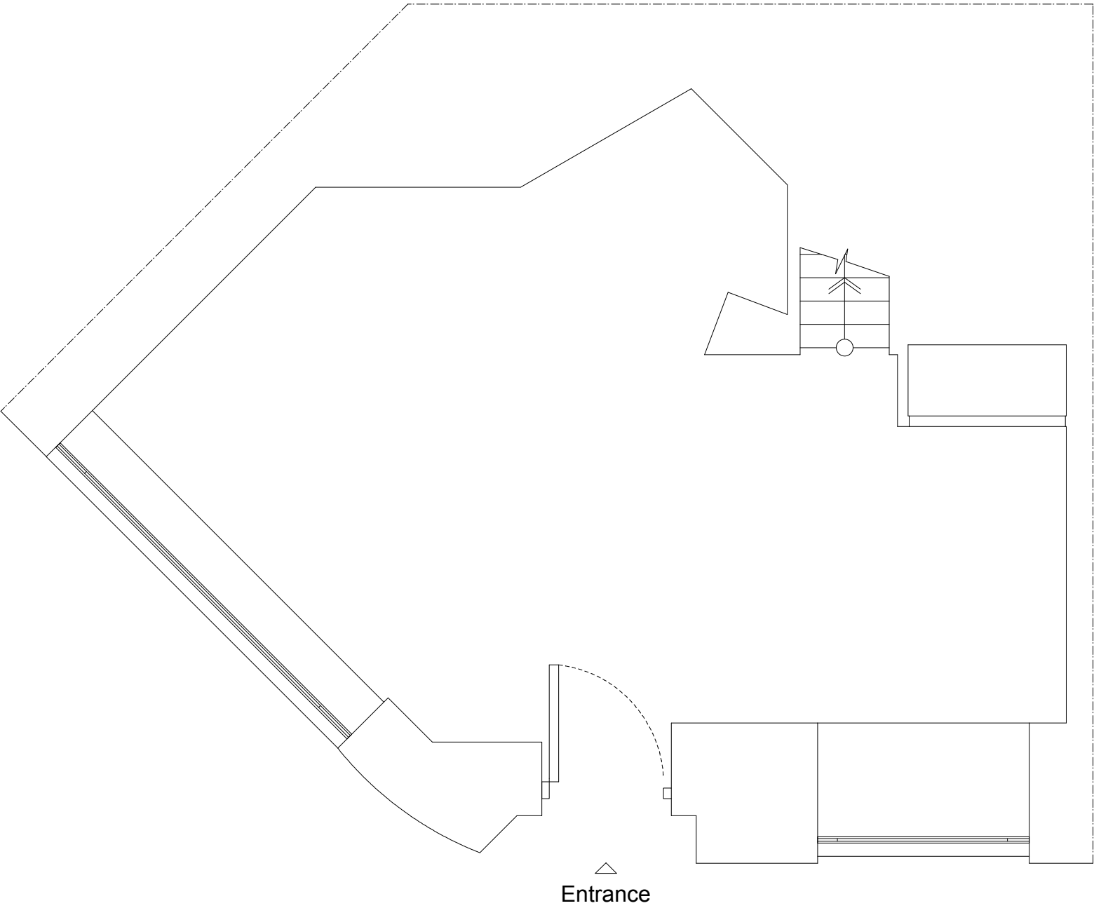
1 103 Plan: Shop Floor Plan: Existing Scale: 1:50 @ A3
