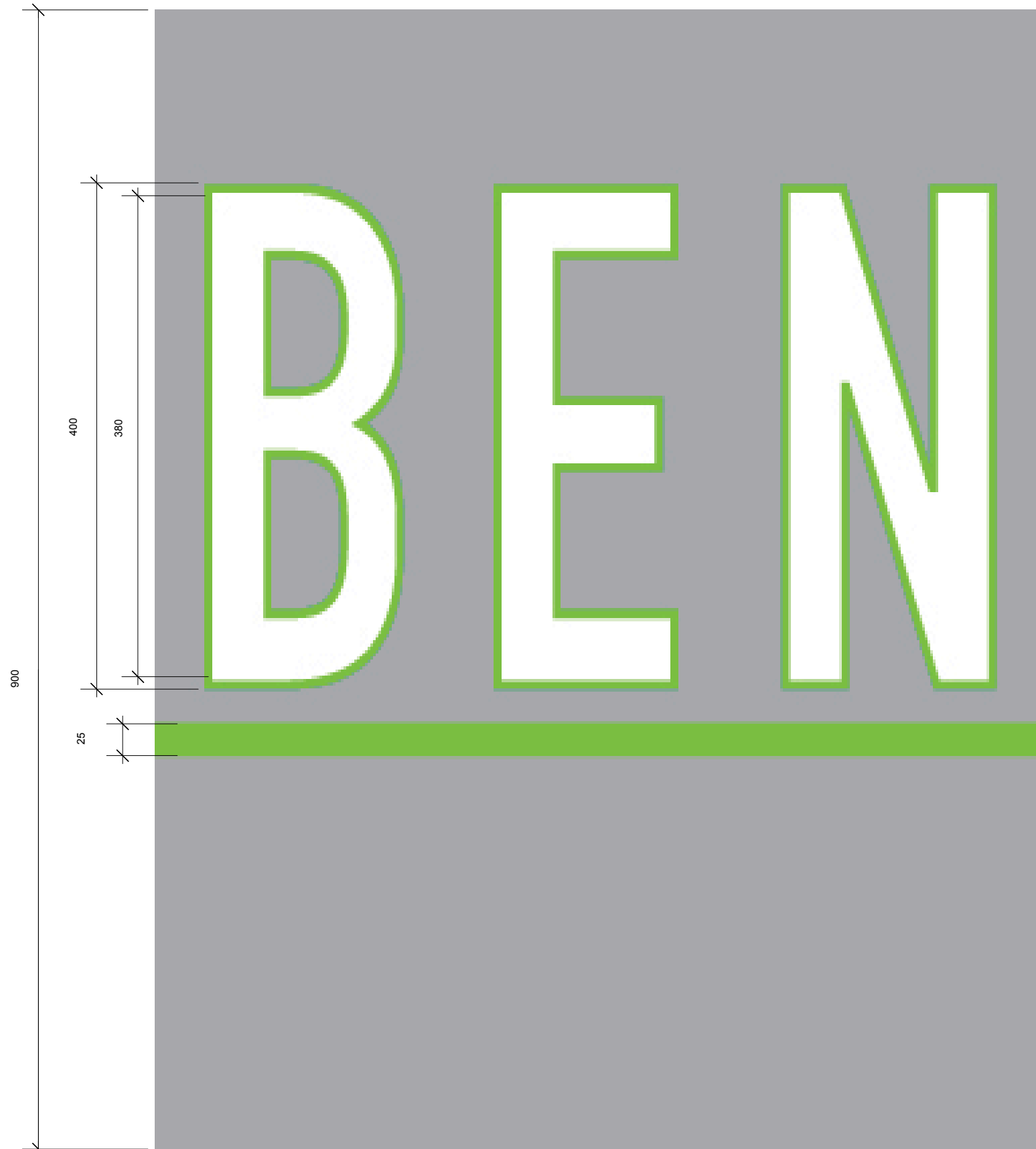
02 PROPOSED FASCIA SIGNAGE ELEVATION 202-02 Scale: 1:4
