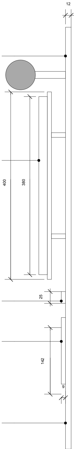
01 PROPOSED FASCIA SIGNAGE SIDE SECTION 202-01 Scale: 1:4
