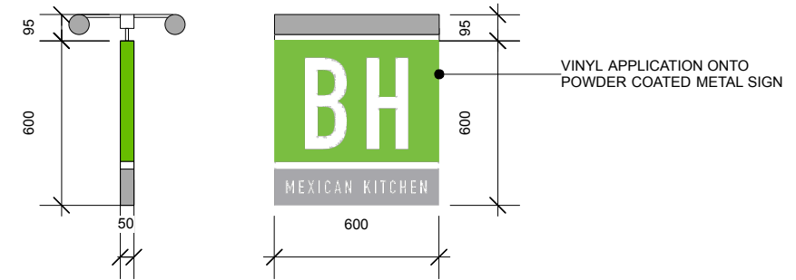
03 PROPOSED PROJECTING SIGN 201-03 Scale: 1:25
