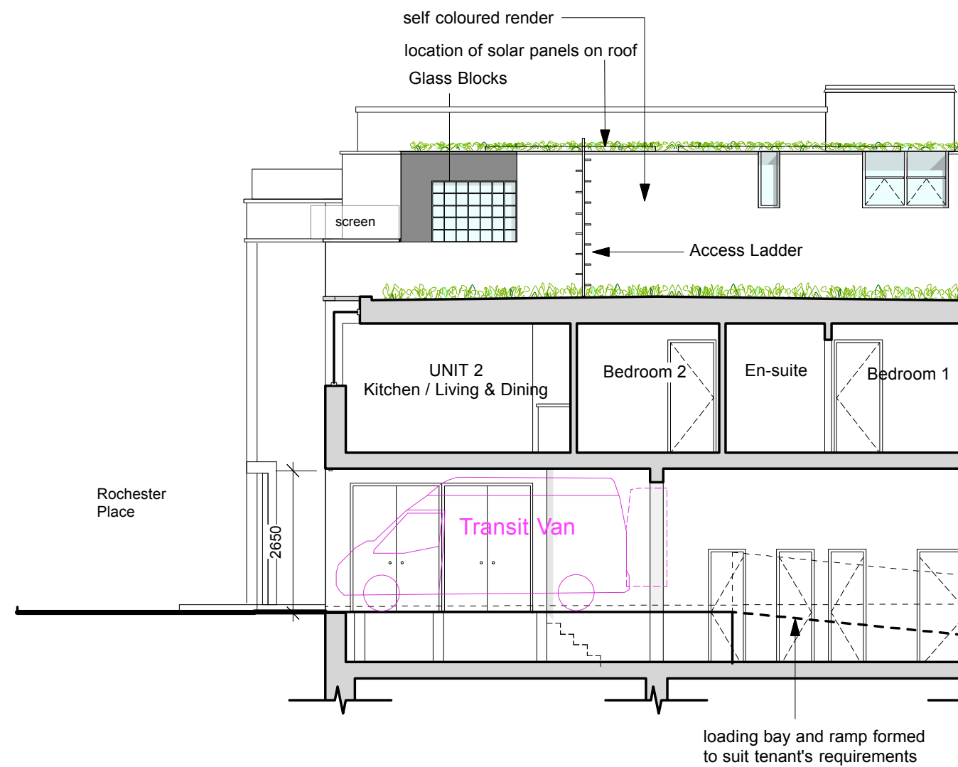
Section Through Loading Bay, Showing Large Transit Van
