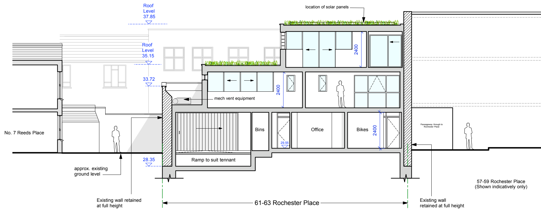
Proposed Section E-E
