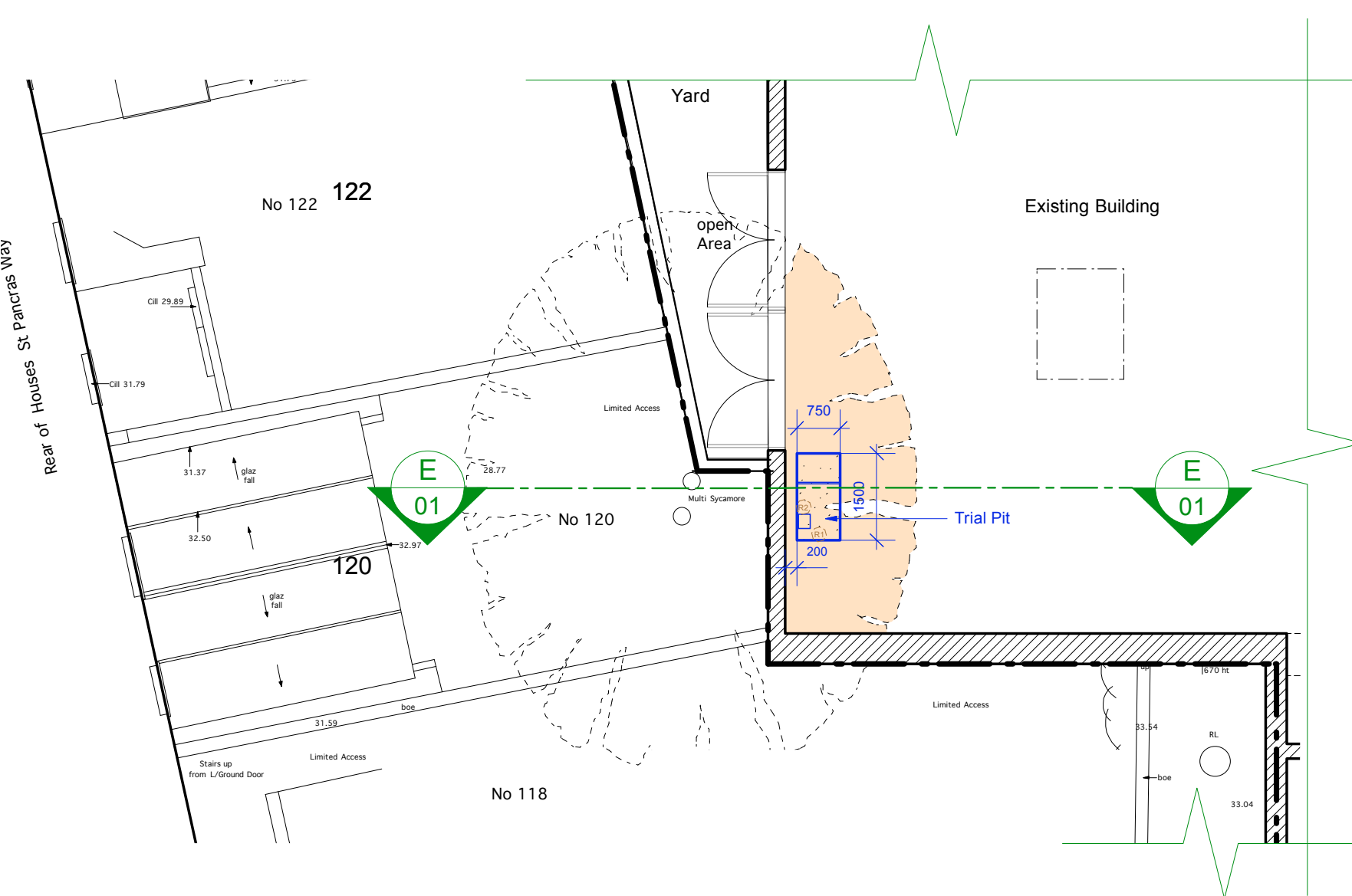
Trial Pit Plan
