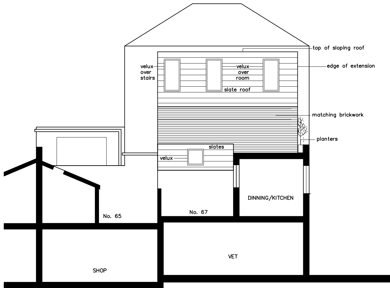
Section CC Proposed
