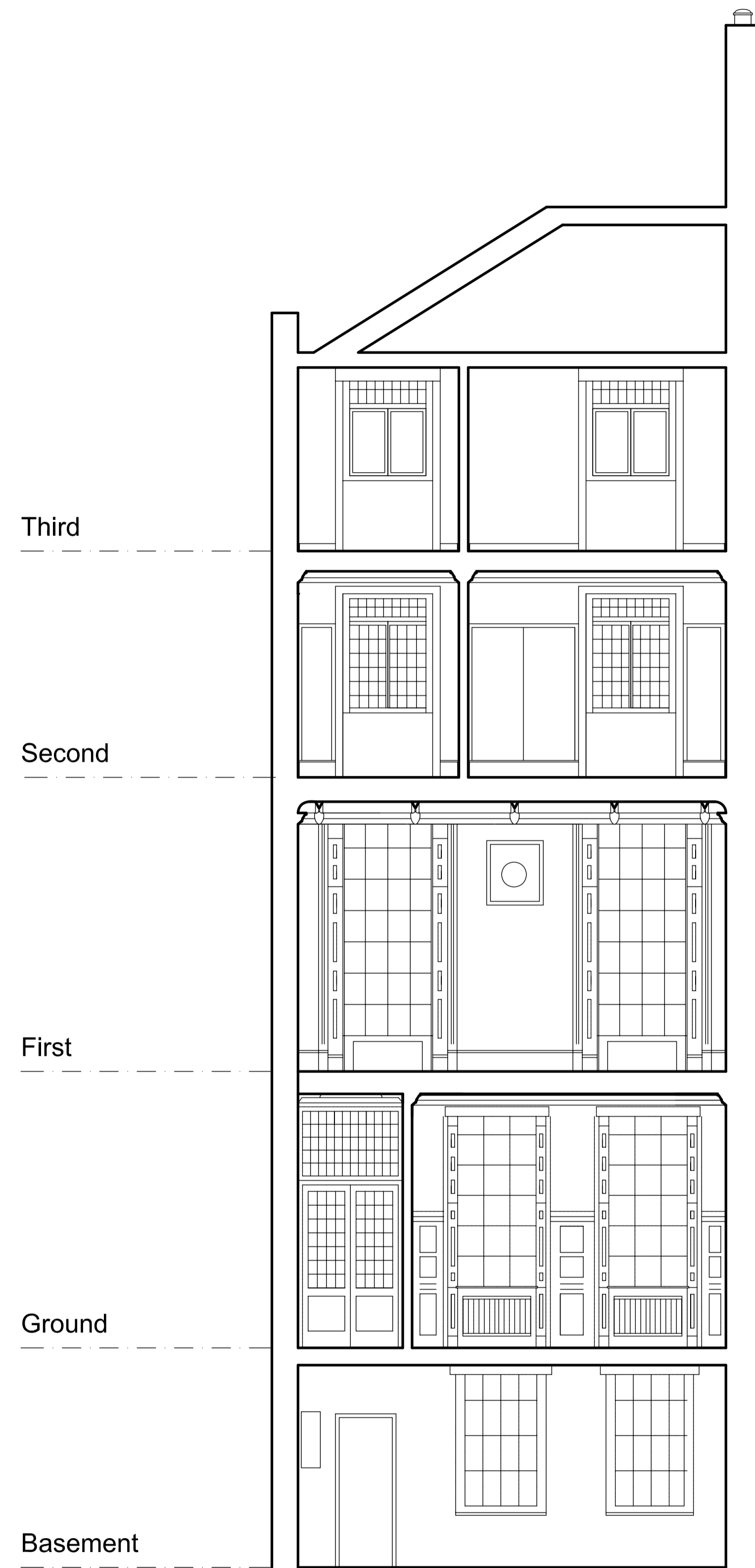
Section CC
