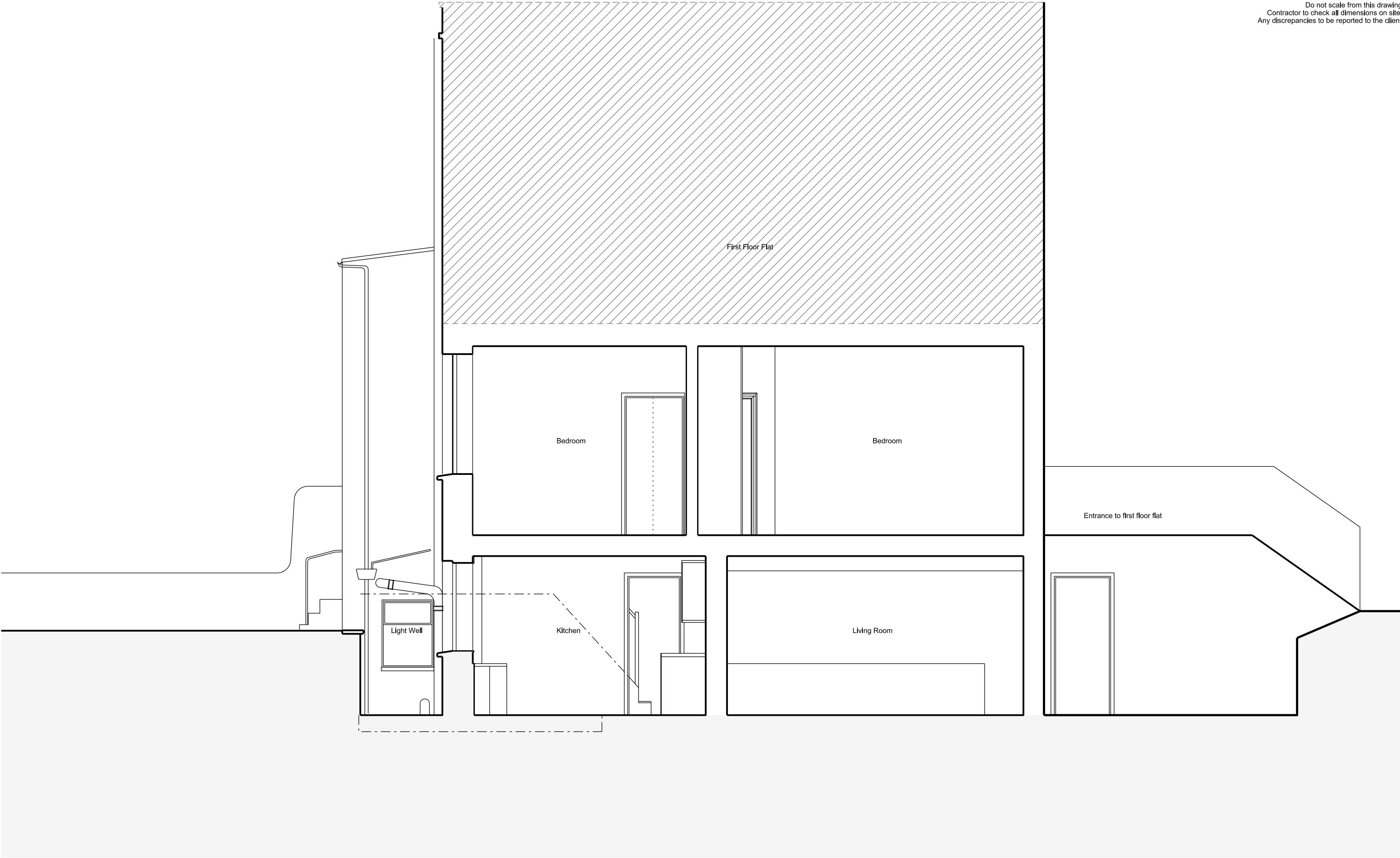
Existing Section AA Scale 1:50 @ A3
