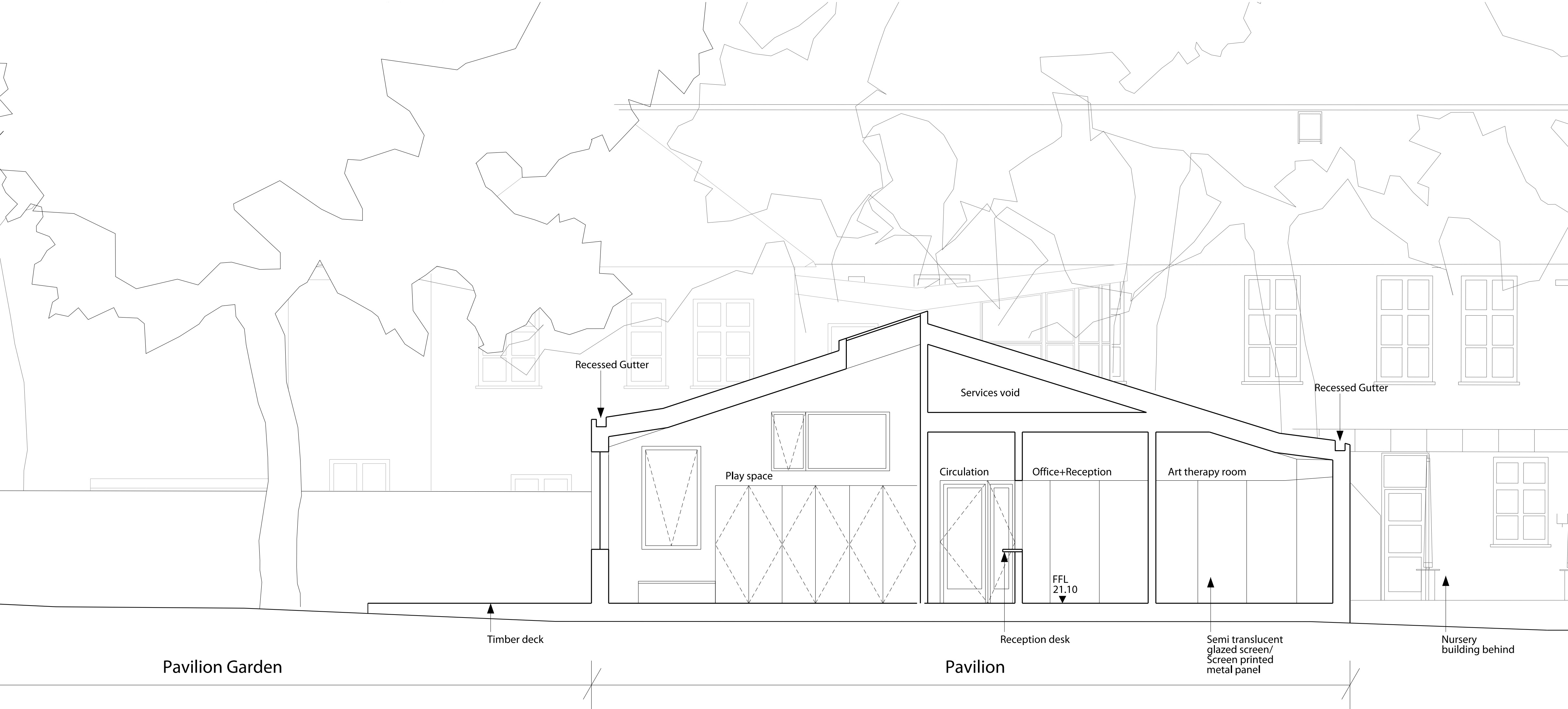
Proposed Section AA
