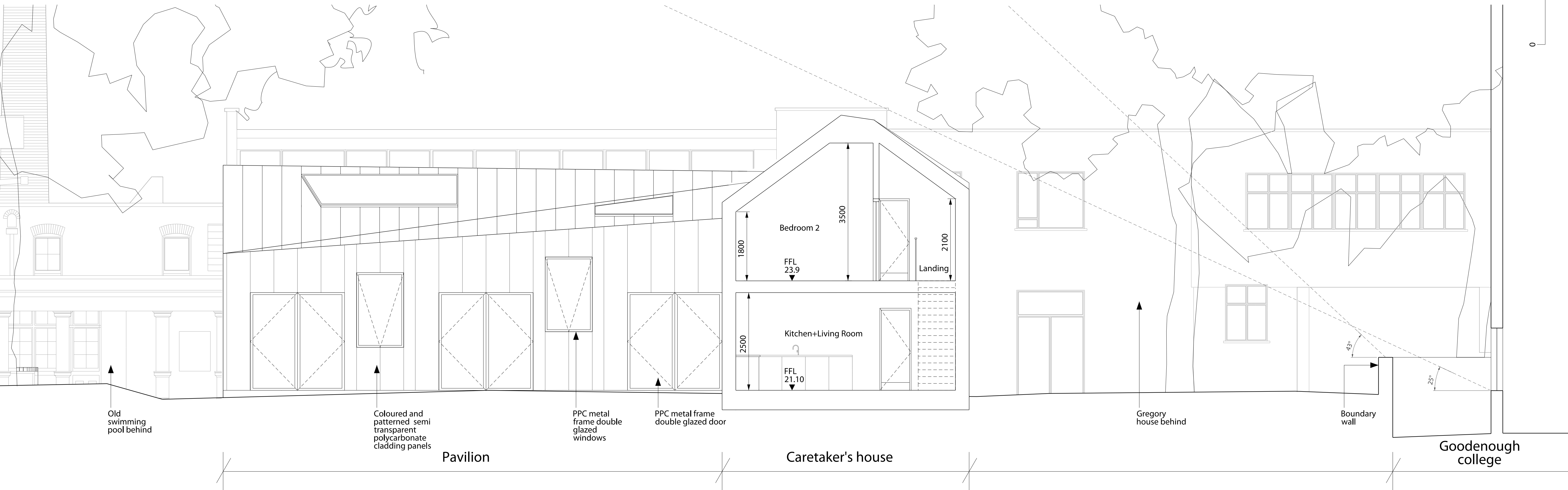
Proposed Section BB
