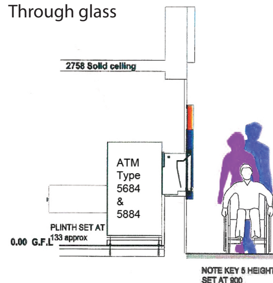
PROPOSED ATM SECTION SCALE (1:50)
