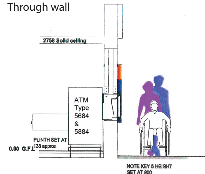
PROPOSED ATM SECTION SCALE (1:50)
