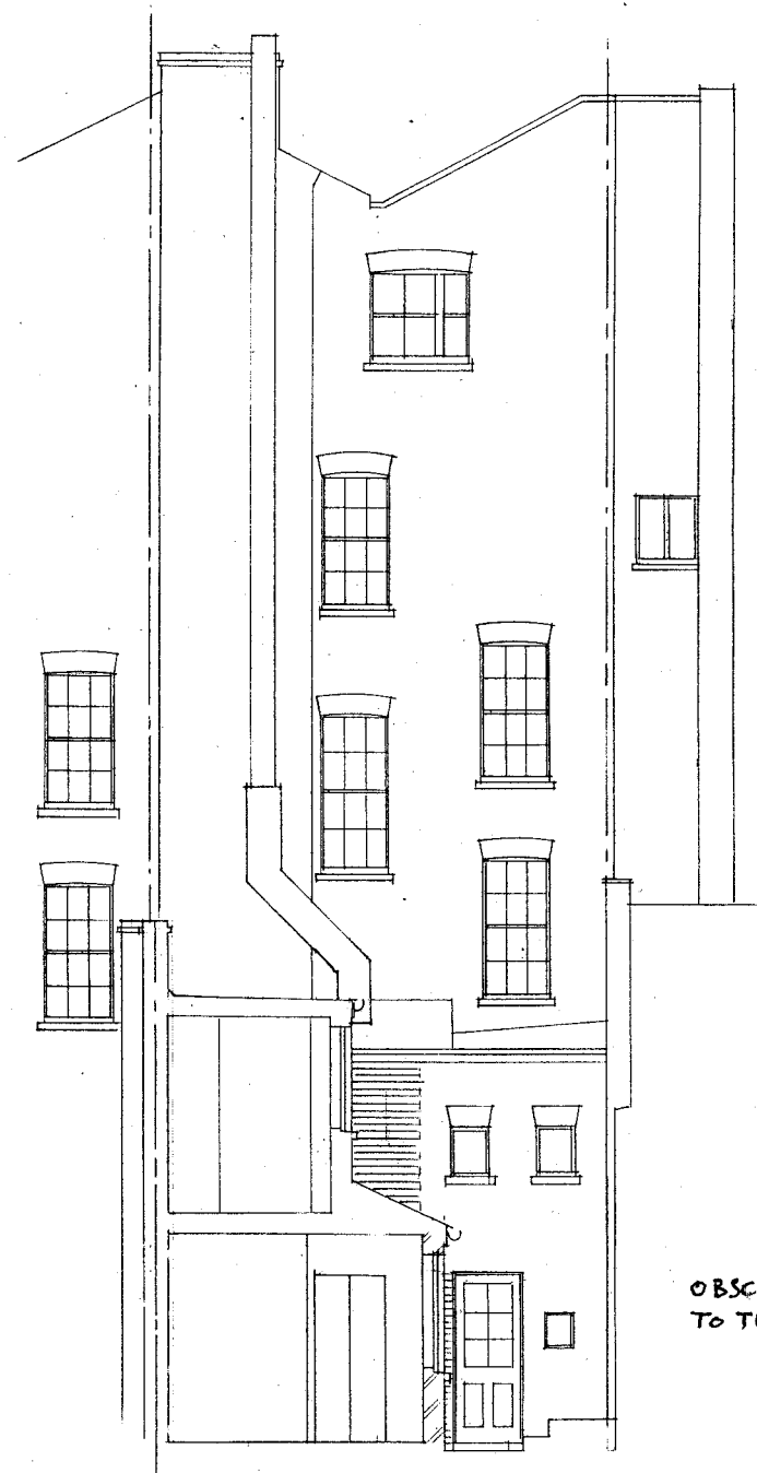
REAR ELEVATION
