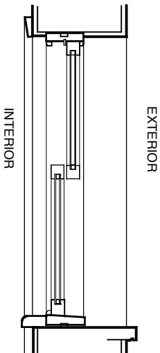
TYPICAL SECTION - BW1, BW2, GW1, GW3
