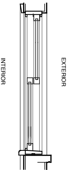
SECTION - GW2
