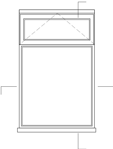
EXTERIOR ELEVATION - BW3, BW4, BW5,GW3
