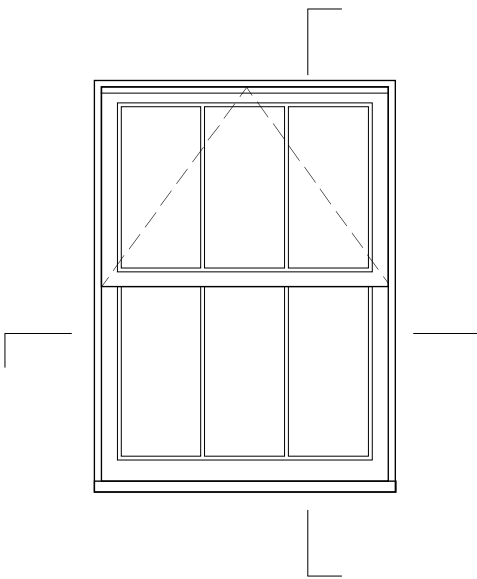
TYPICAL EXTERIOR ELEVATION - BW1, BW2, GW1, GW3
