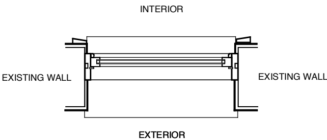
TYPICAL PLAN - BW1, BW2, GW1, GW3
