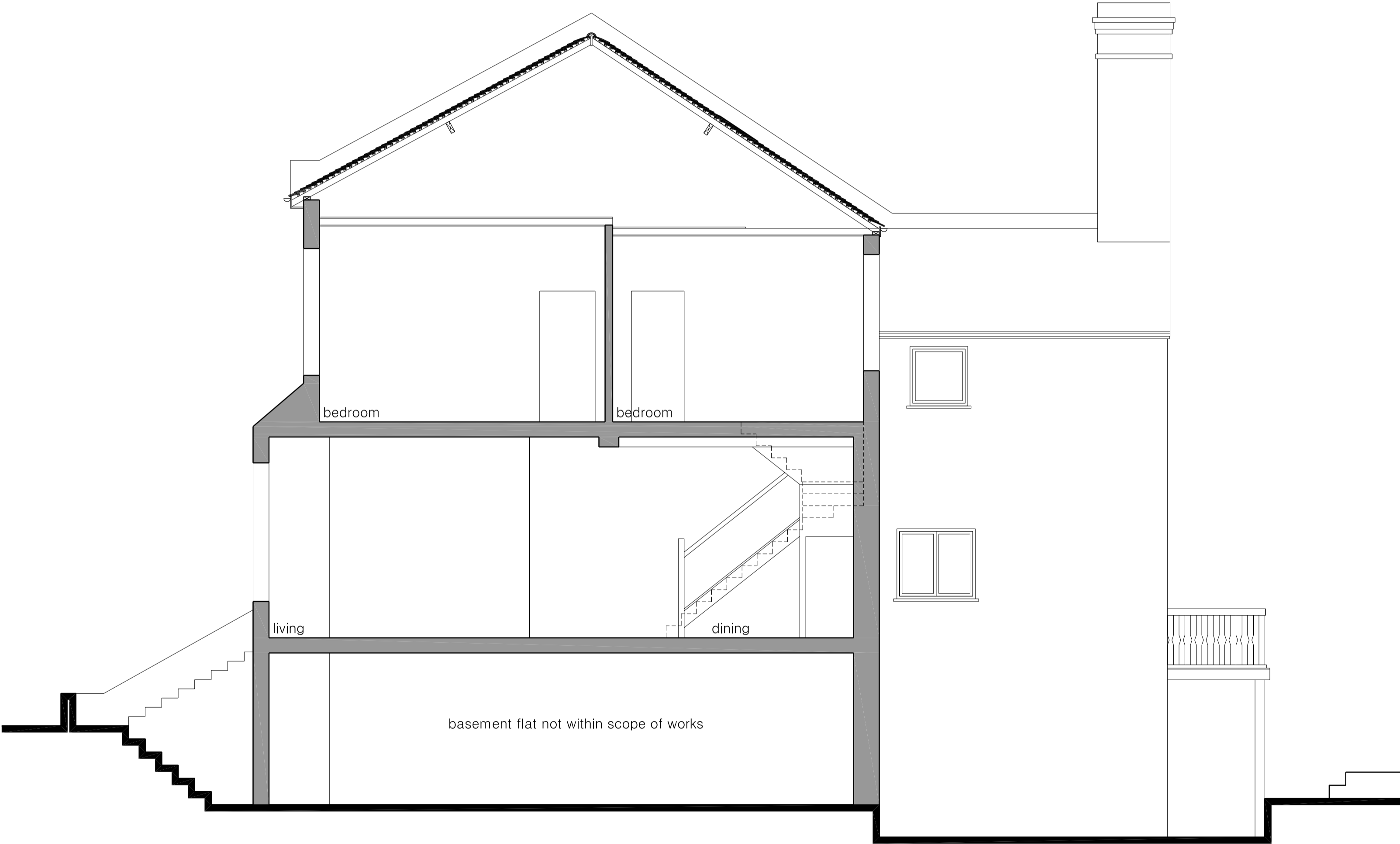
section A-A existing
