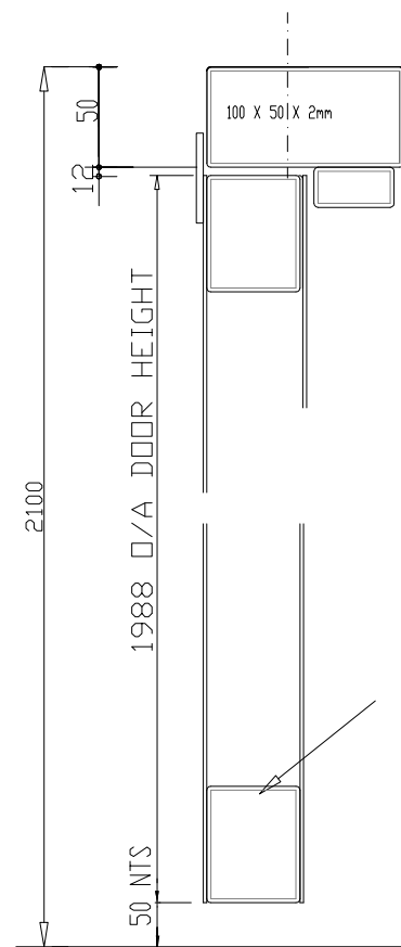
HEIGHT SECTION THRO' DOORSET
