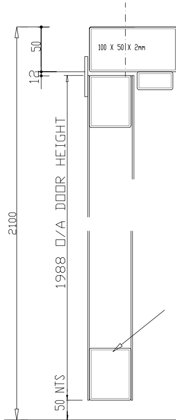
HEIGHT SECTION THRO' DOORSET
