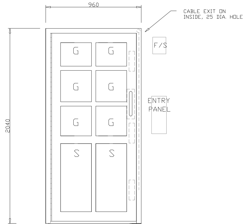
ELEVATION OF TYPICAL SINGLE DOORSET HLOO NB. DOOR DRAWN OPENING OUT TOWARDS VIEWER
