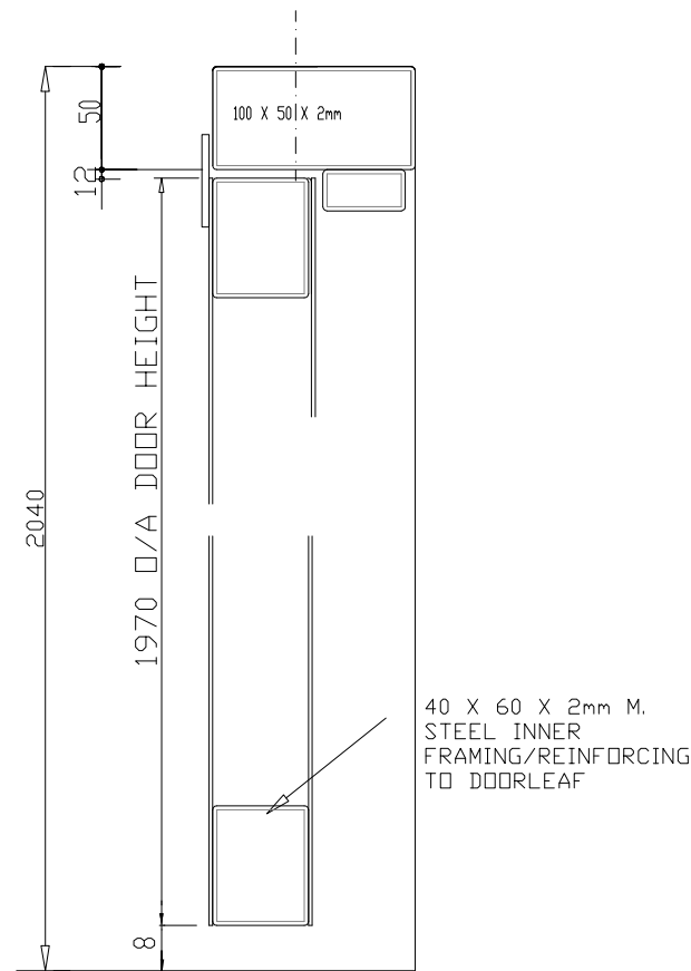
HEIGHT SECTION THRO' DOORSET
