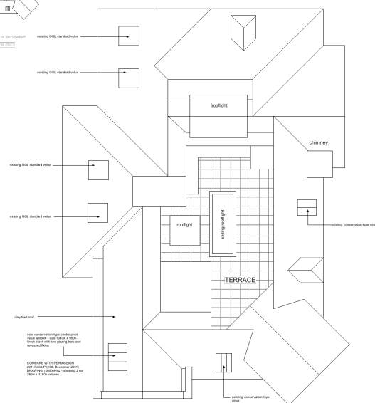
ROOF PLAN - PROPOSED
