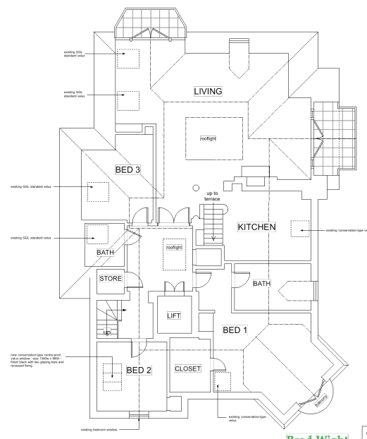
SECOND FLOOR - FLAT 4 - PROPOSED
