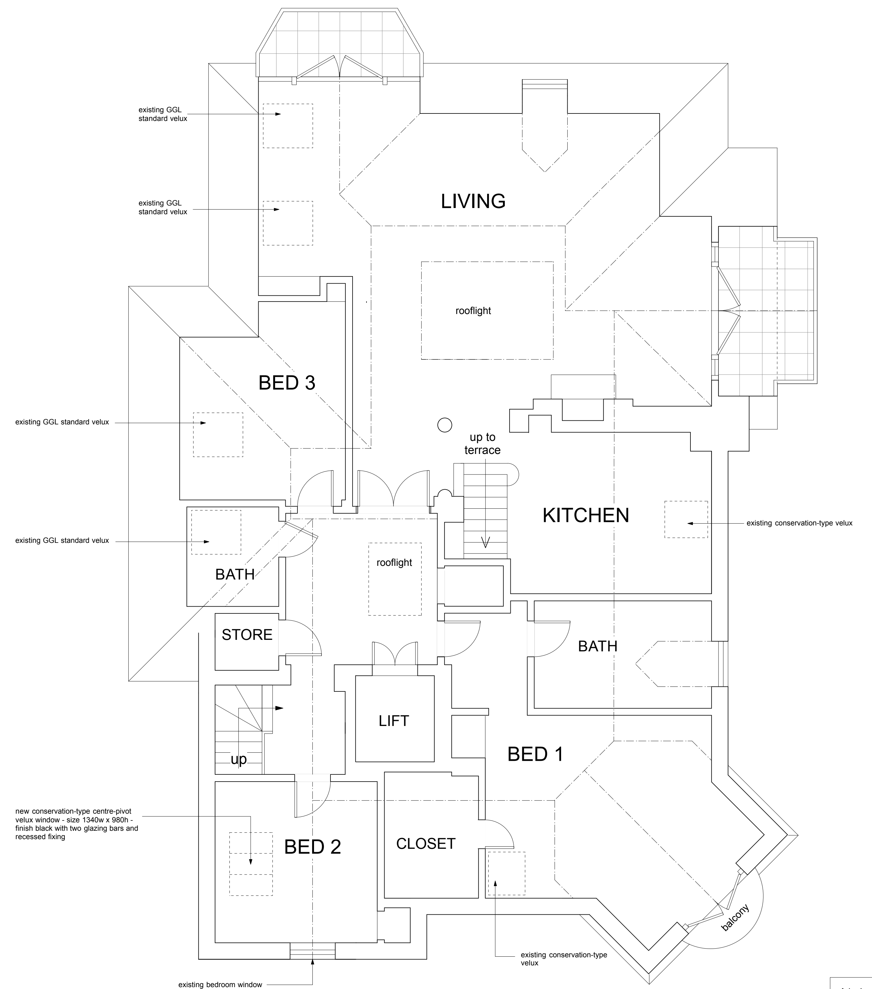
SECOND FLOOR - FLAT 4 - PROPOSED
