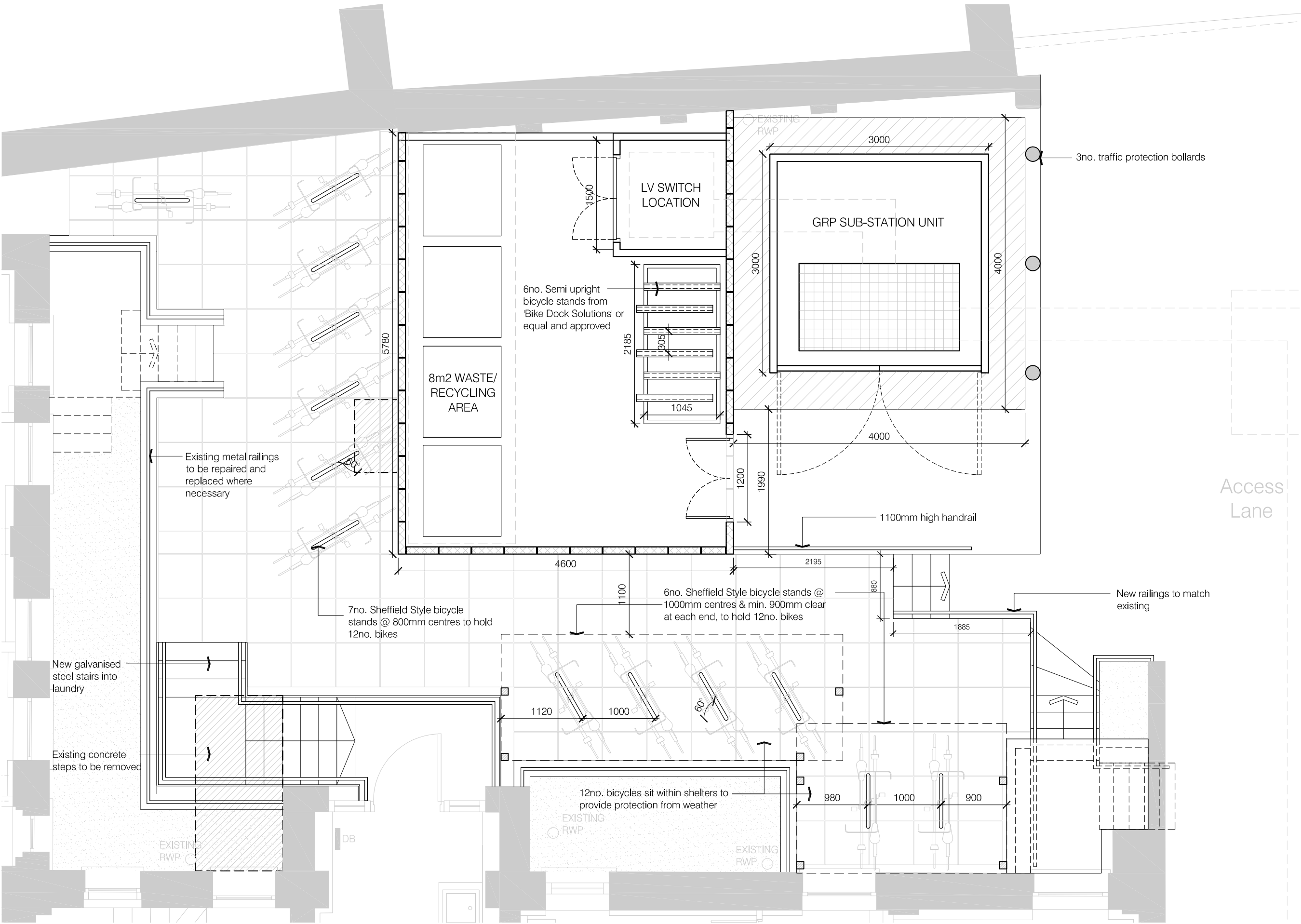
Courtyard Layout Scale: 1:50
