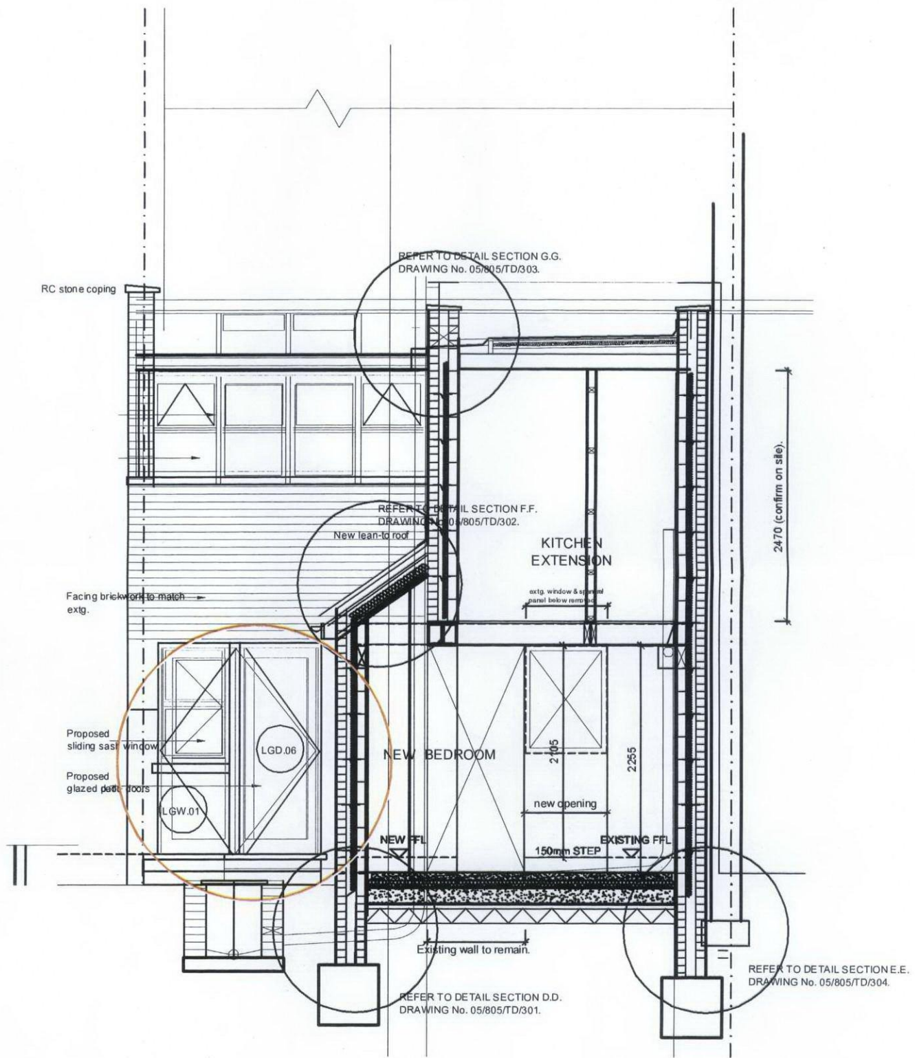
Section C-C
