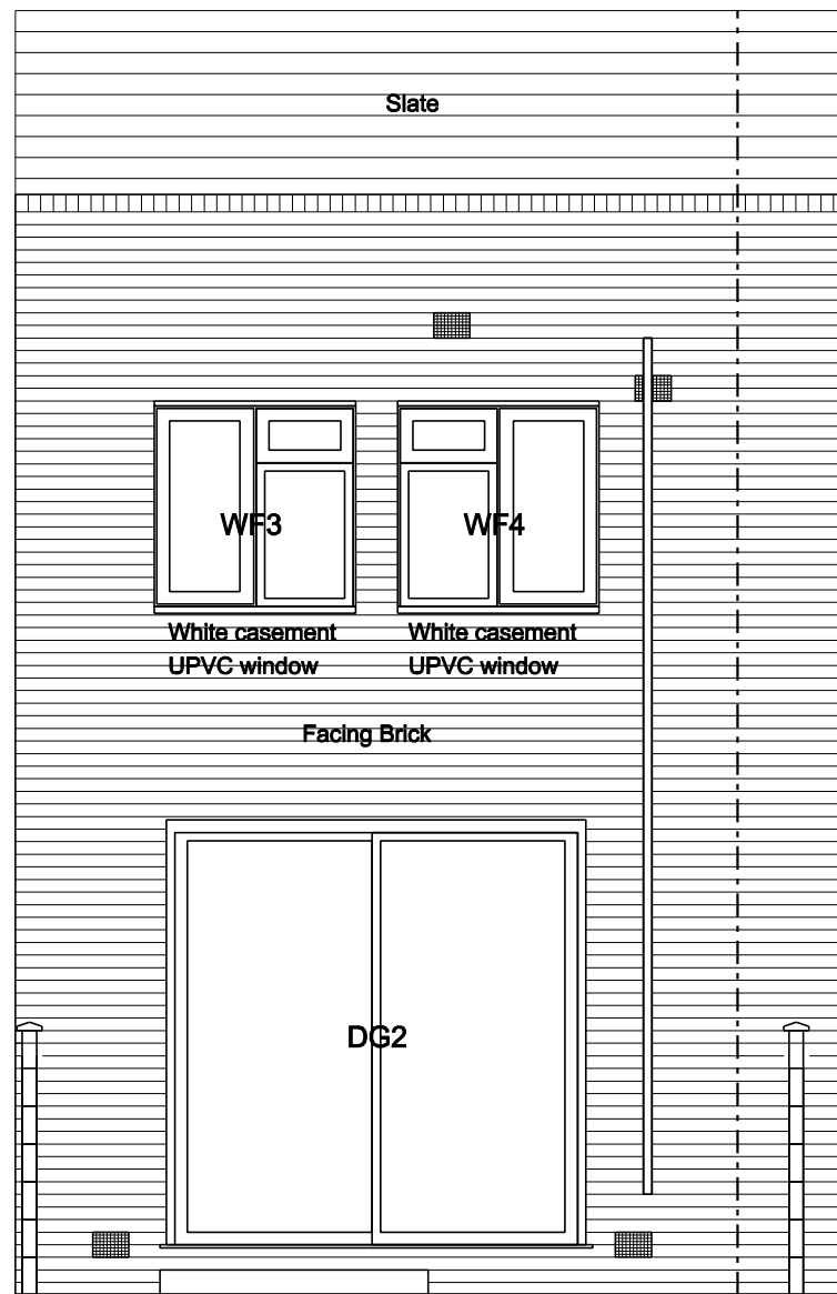
REAR ELEVATION
