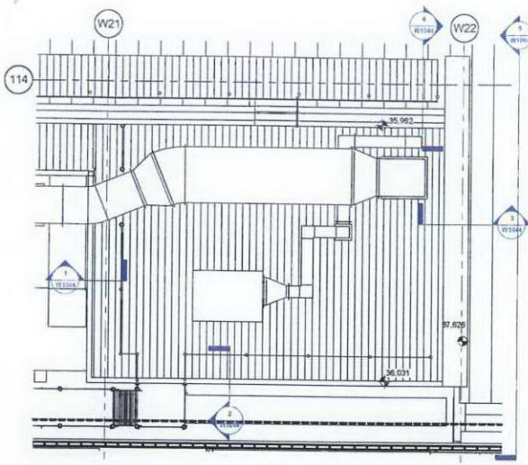
A Core 4 Roof 1:50
