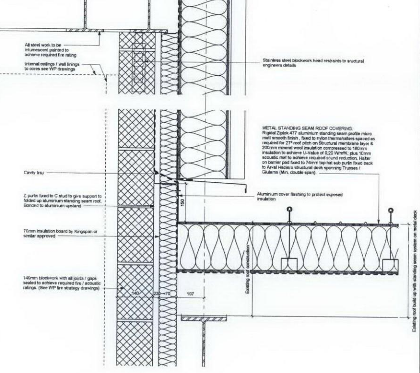
3 Core 4 Roof Section 3 1:5
