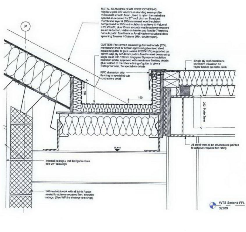
4 Core 4 Roof Section 4 1:5
