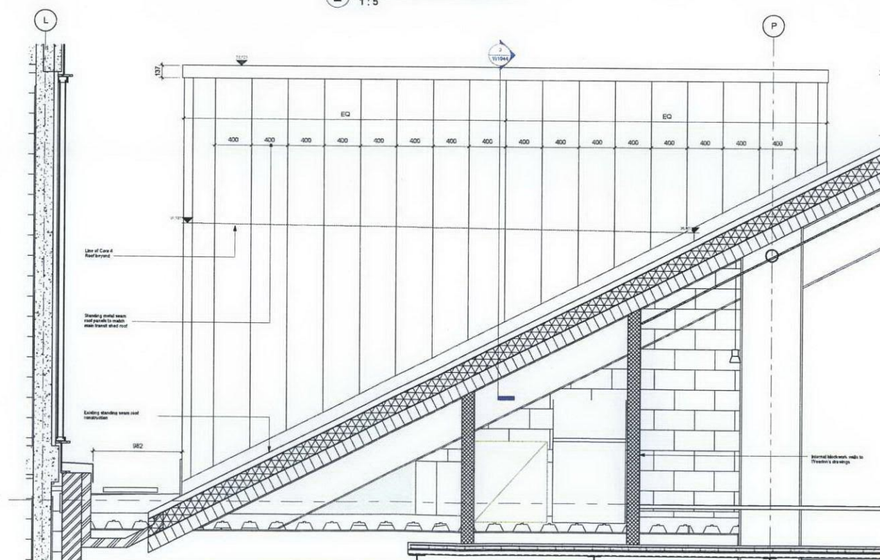
5 Core 4 Roof Side Elevation 1:20
