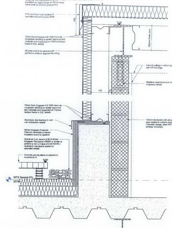
2 Core 4 Roof Section 2 1:5
