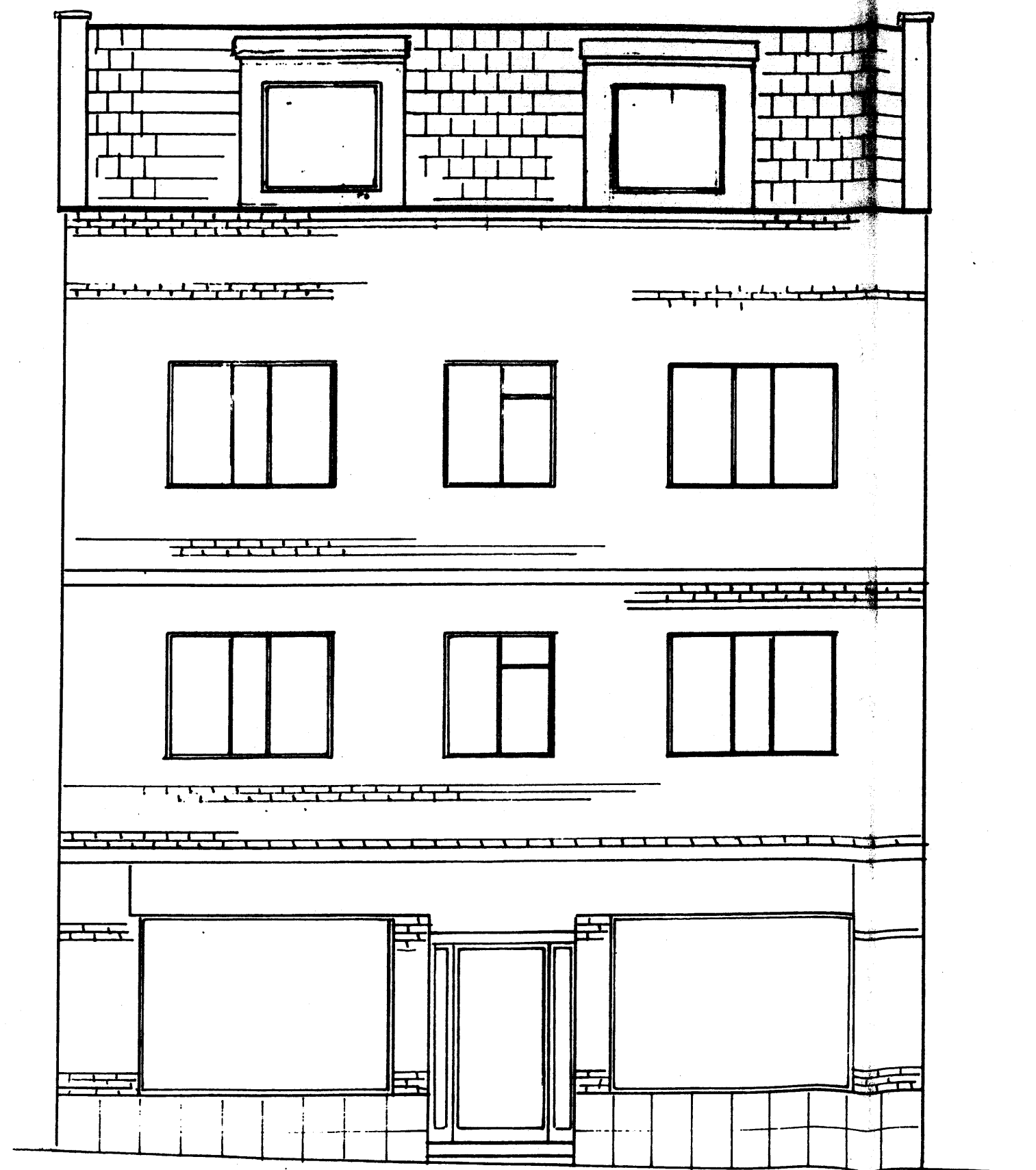
NORTH EAST ELEVATION / FRONT / SCALE 1:50
