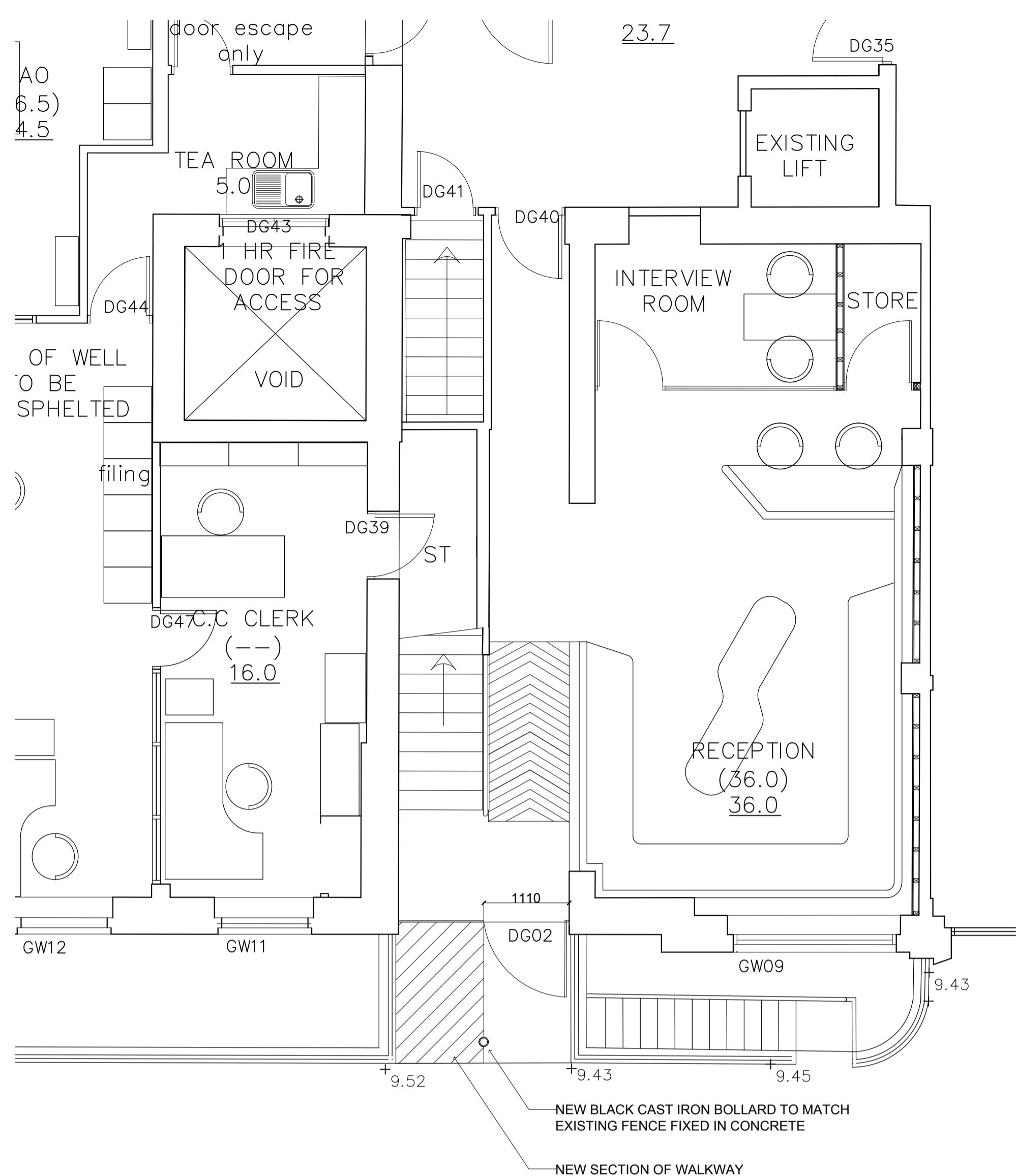
PLAN - NEW ENTRANCE 1:50 @ A1
