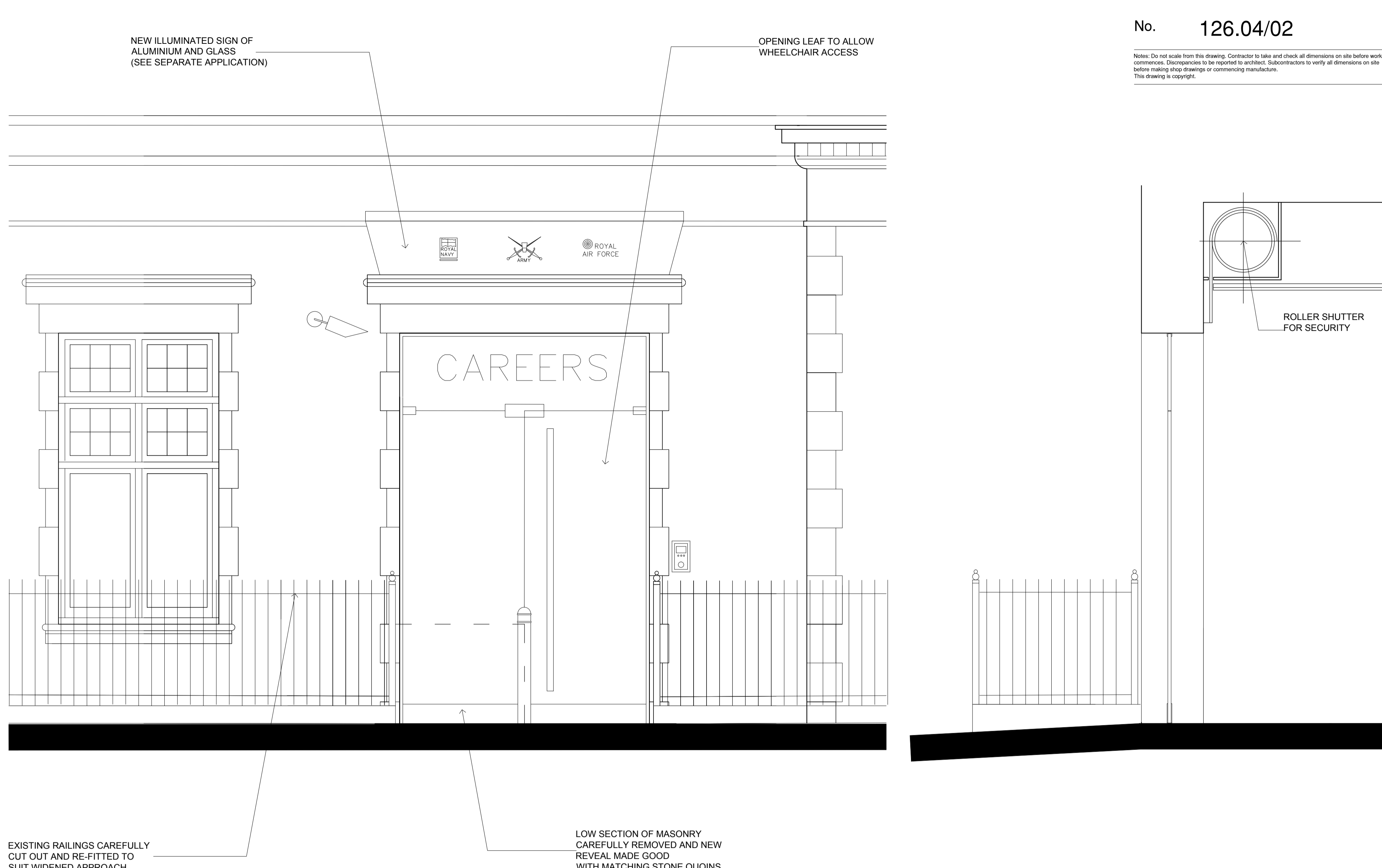
DETAIL A- ELEVATION OF NEW ENTRANCE 1:20 @ A1
