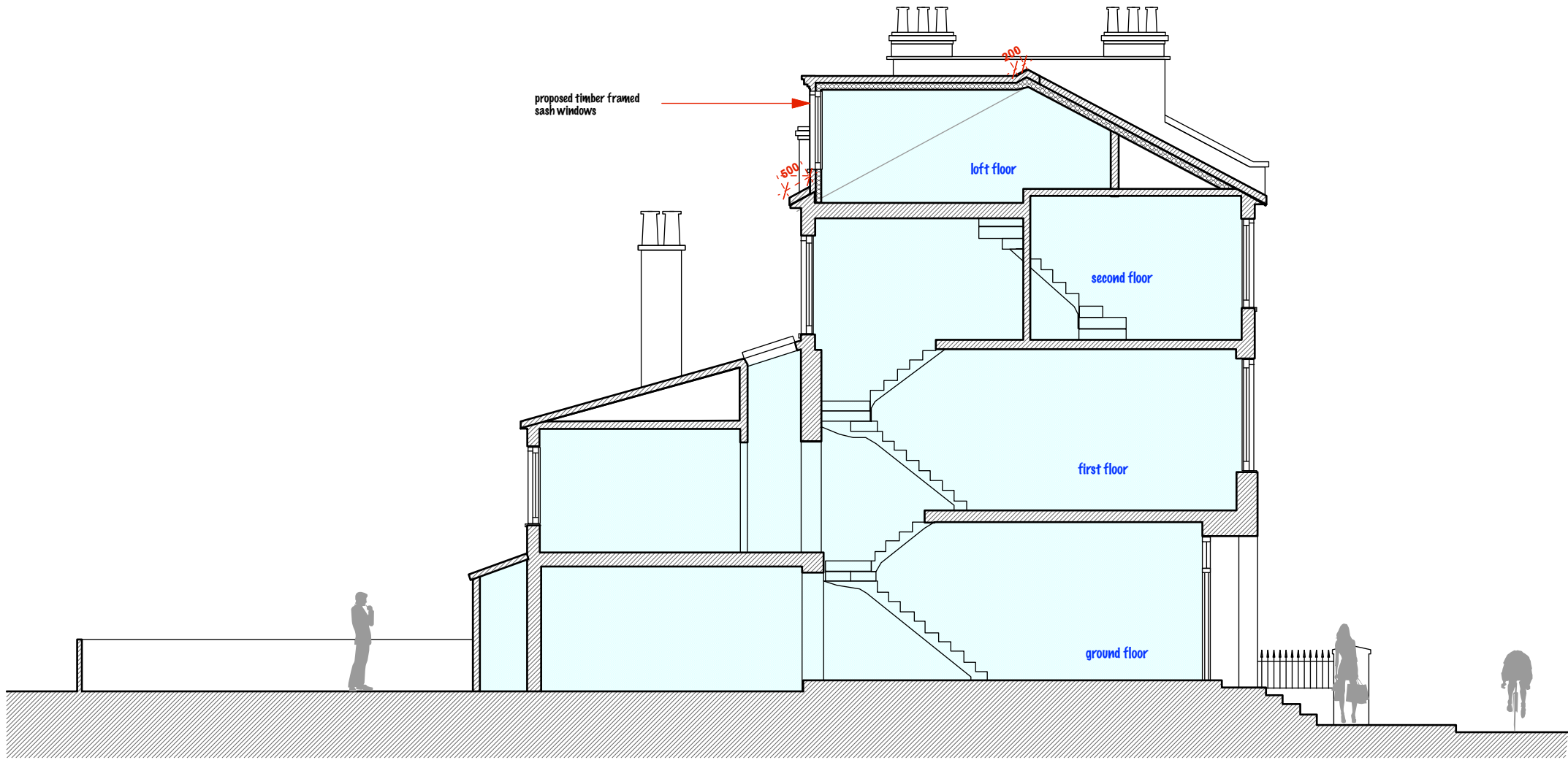
SECTION AA
