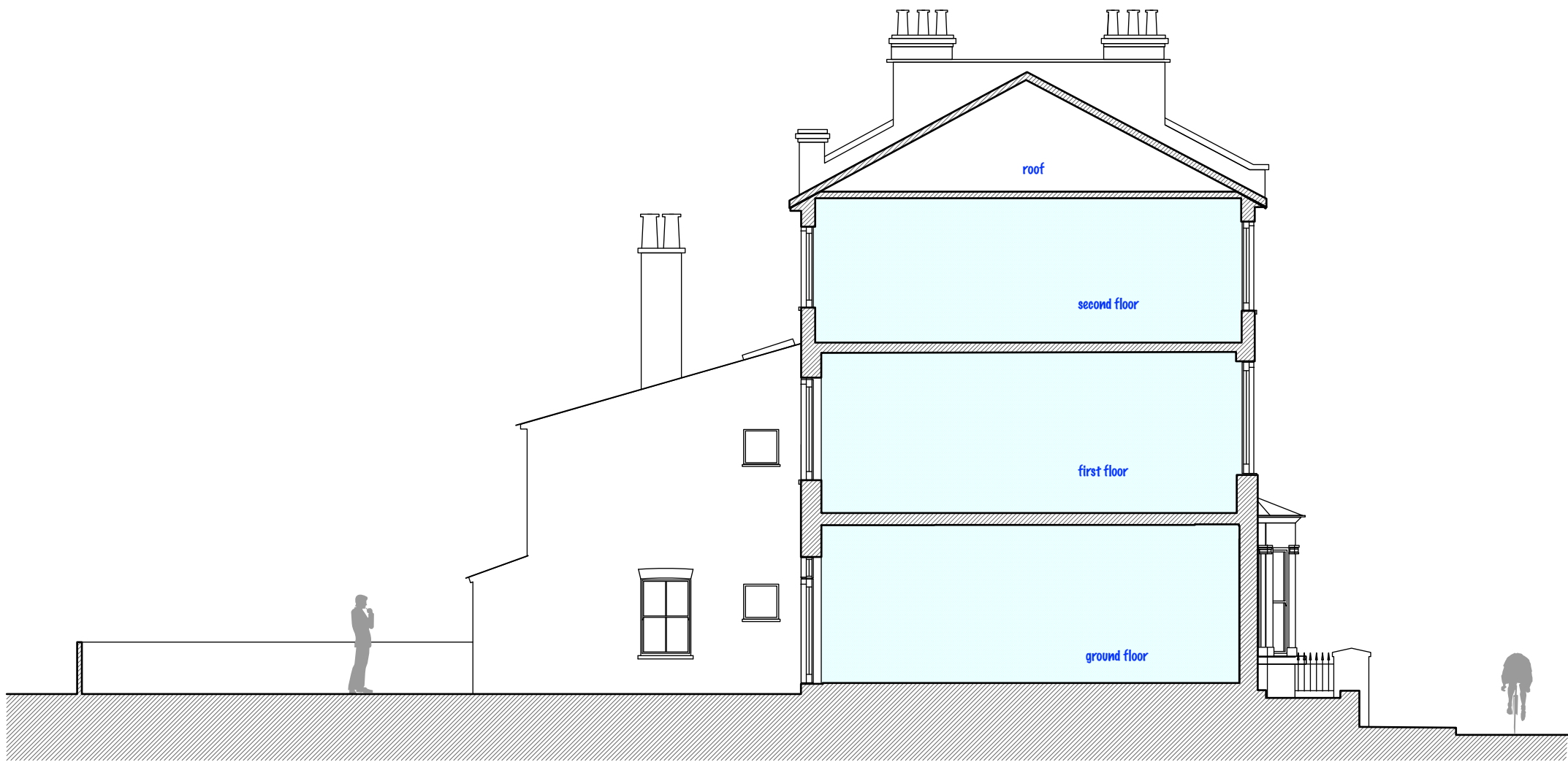
SECTION BB
