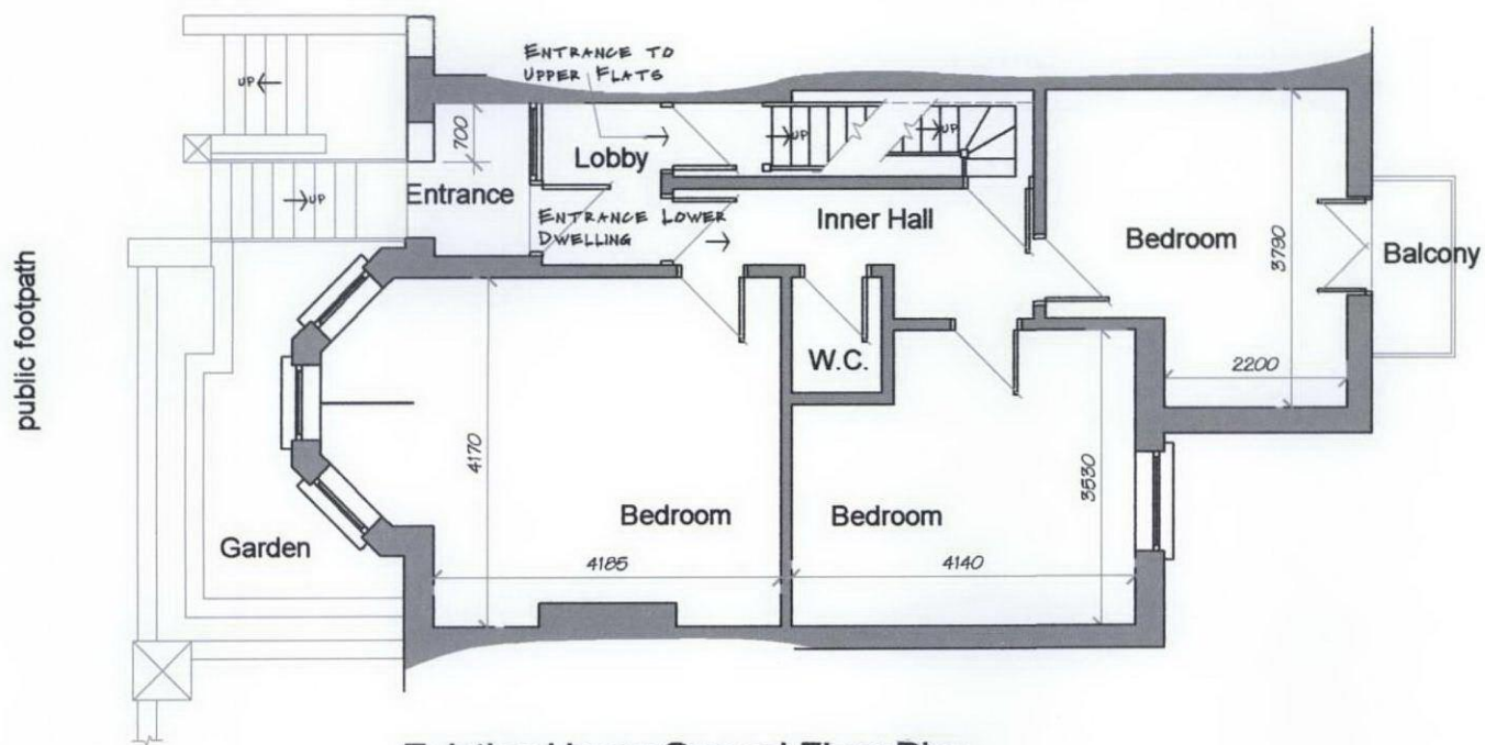
Existing Upper Ground Floor Plan.
