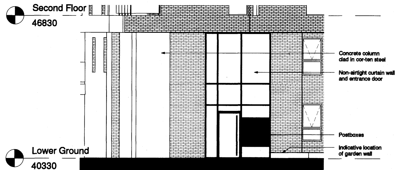
2 0111 Entrance Elevation / Proposed Amendments 1:100
