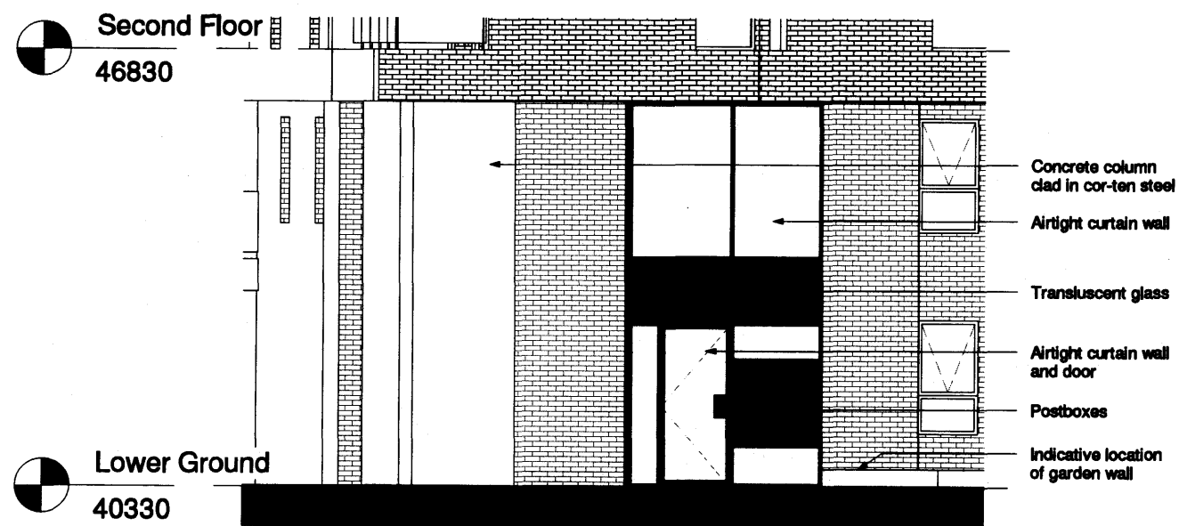
1 0111 Entrance Elevation / Consented Scheme 1:100
