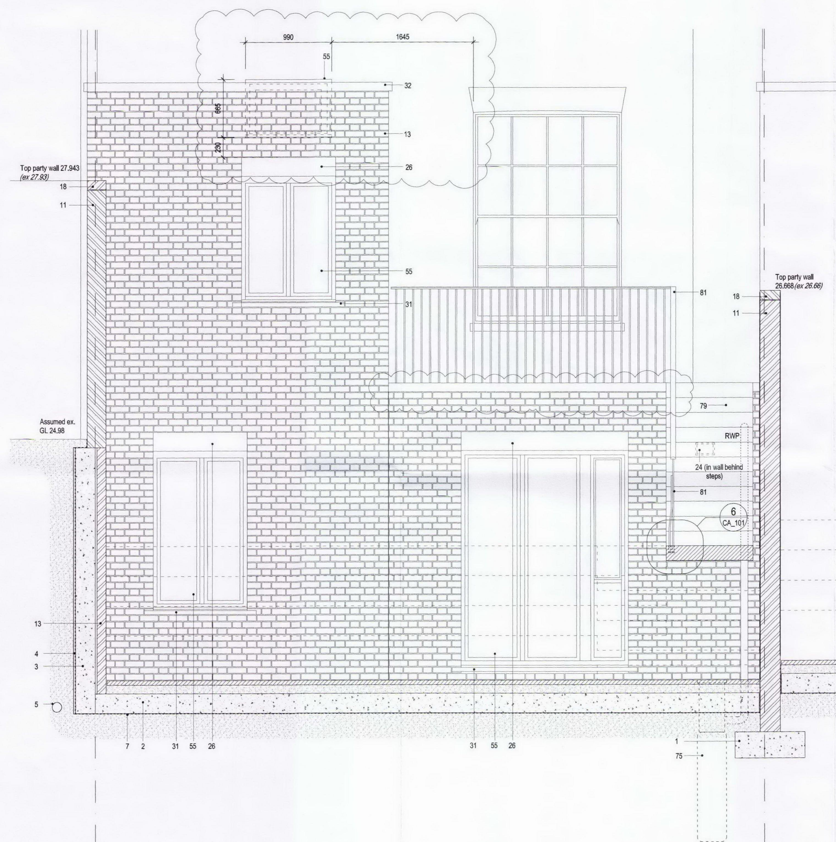
H EL_104 Detail Elevation H
