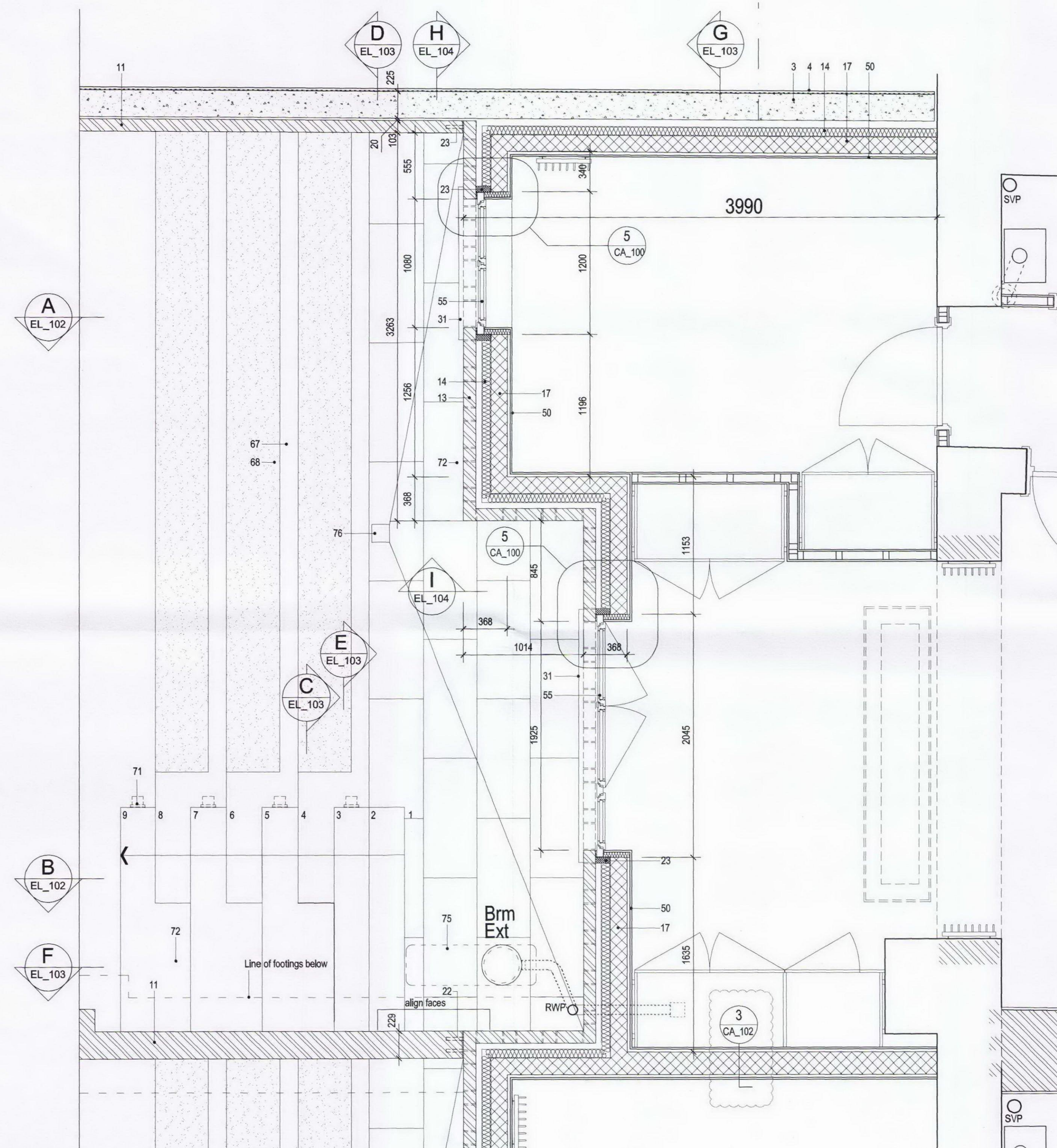
1 EL_101 Detail Plan - Lower Ground Floor
