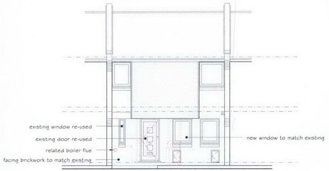
West Elevation - as proposed
