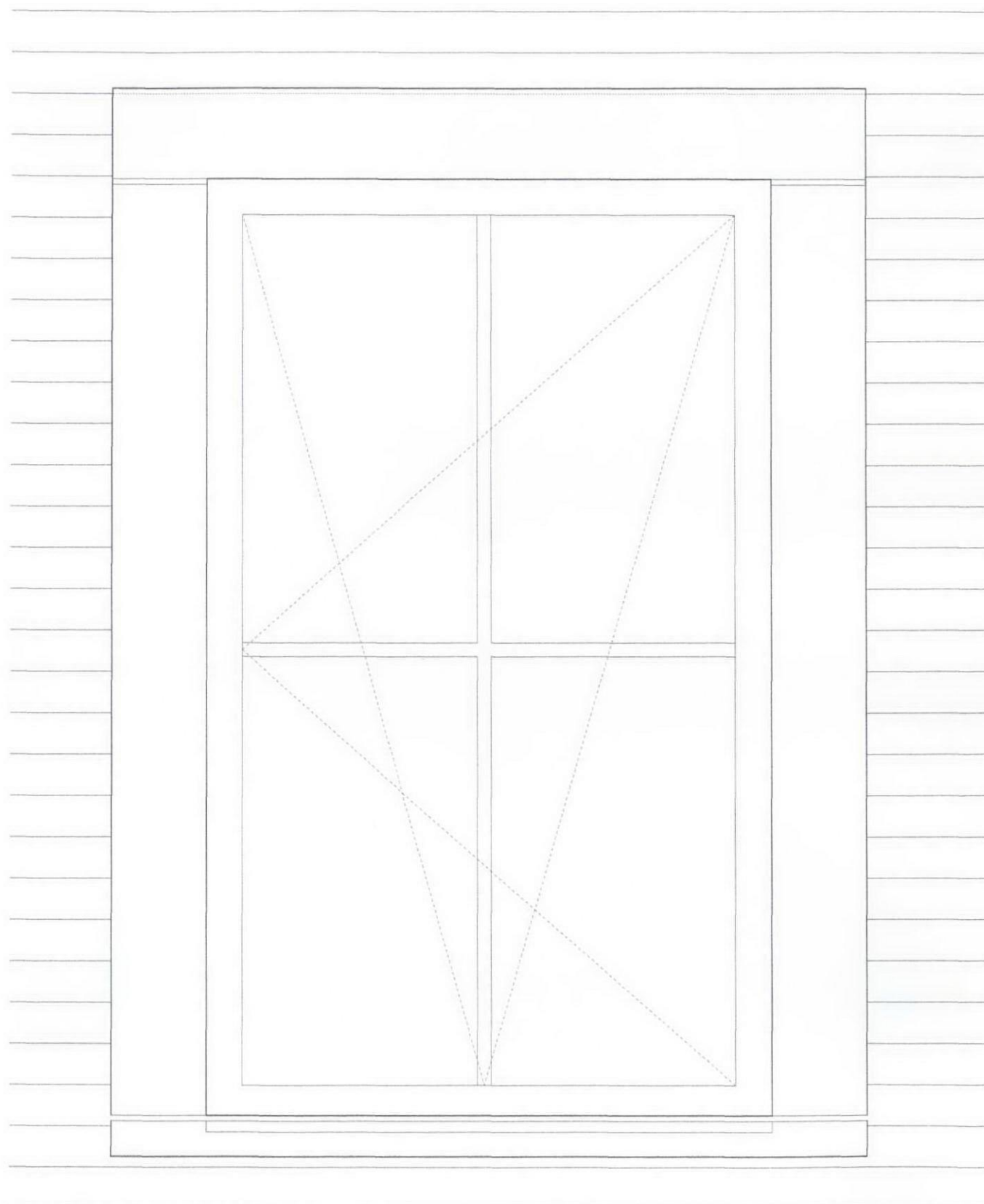
01 1:10 Elevation of second floor window
