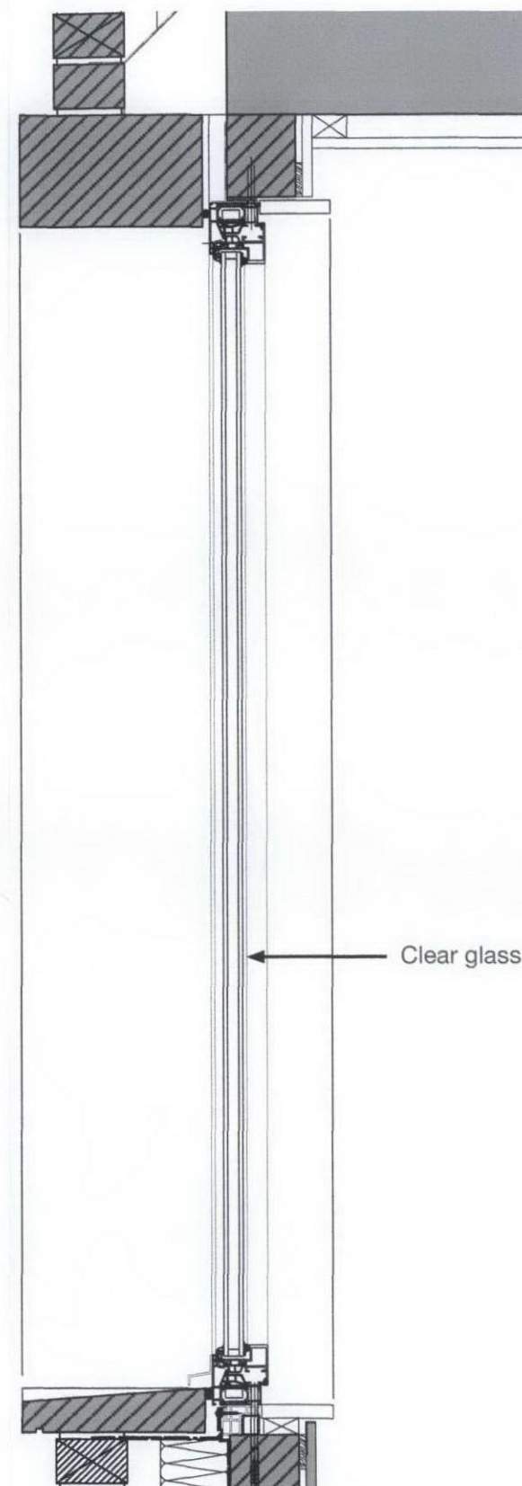
02 1:10 Section through second floor window
