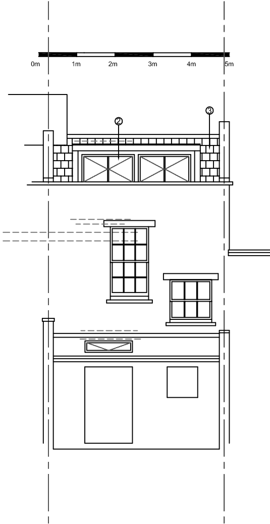
REAR ELEVATION
