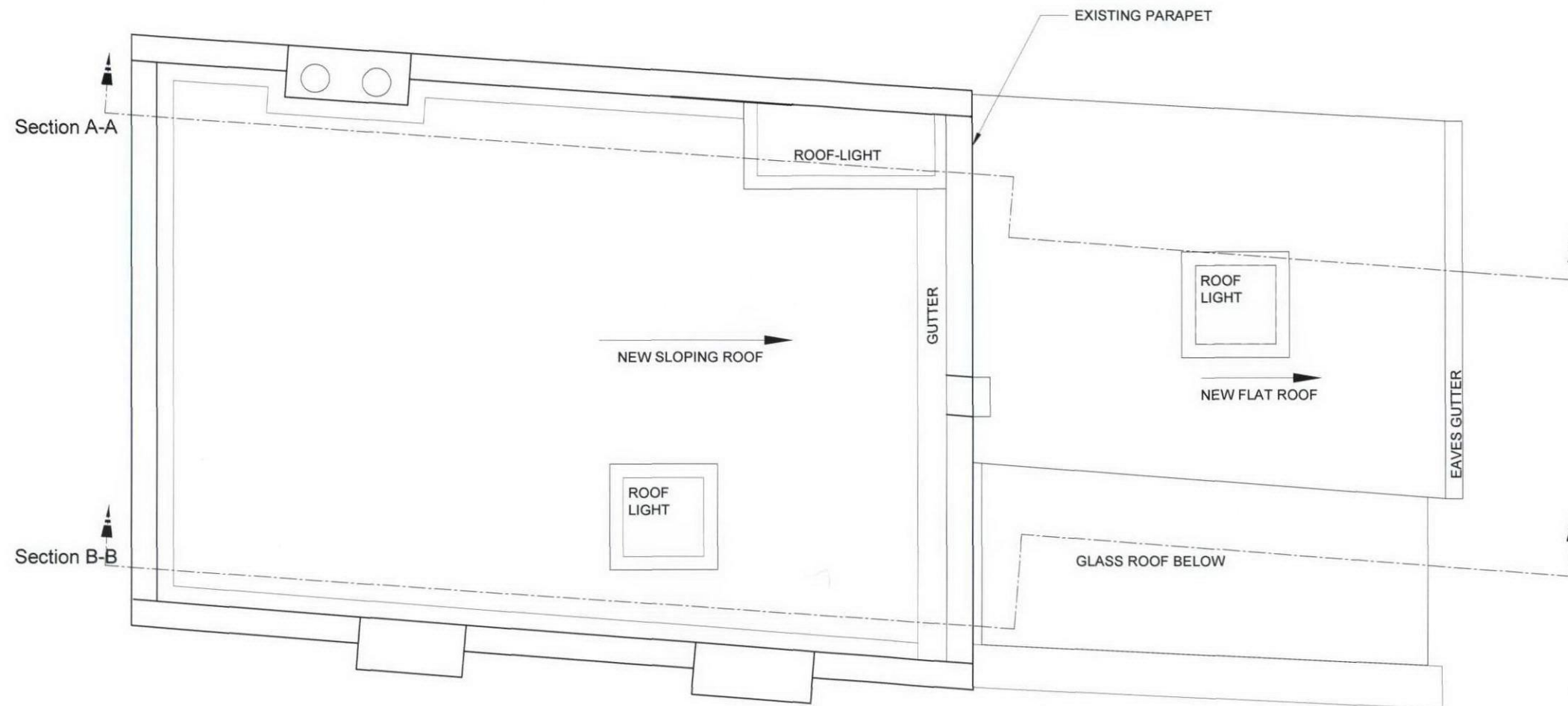
Roof Plan - Proposed
