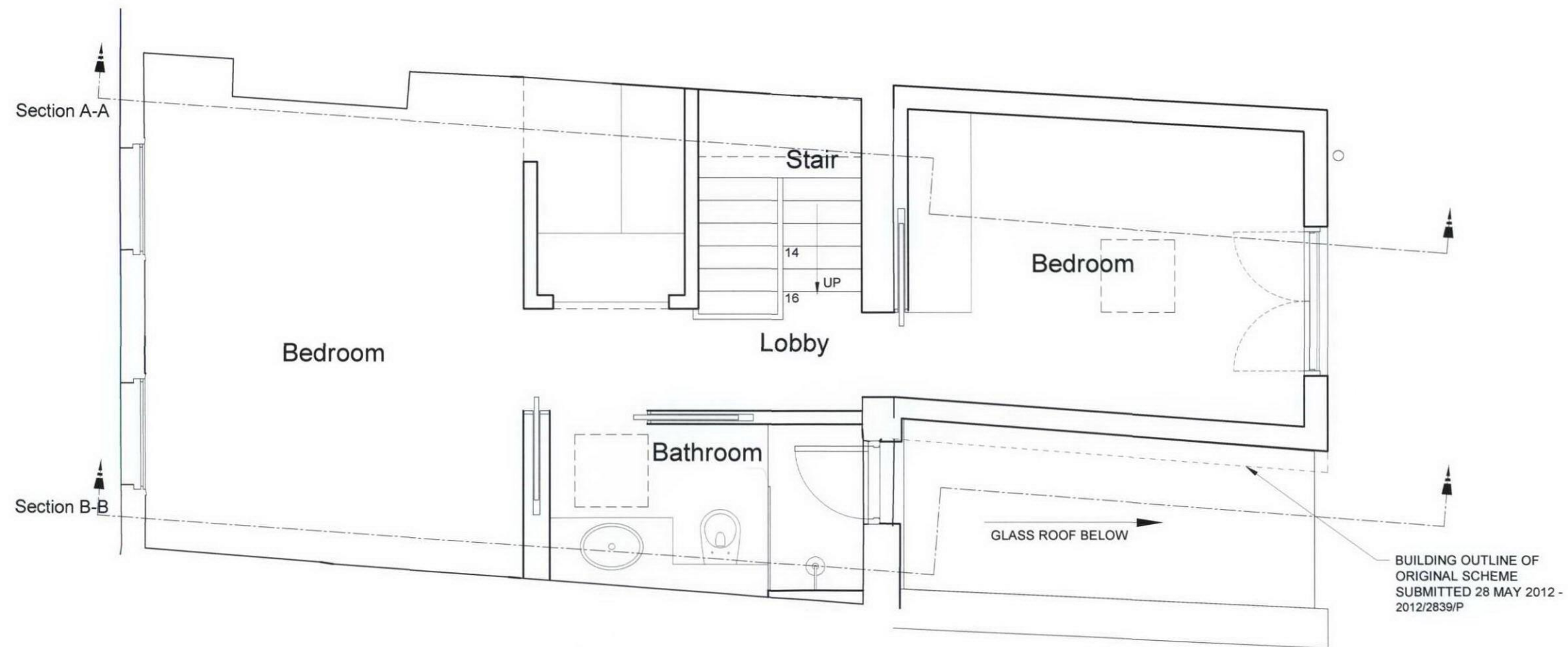
First Floor Plan - Proposed
