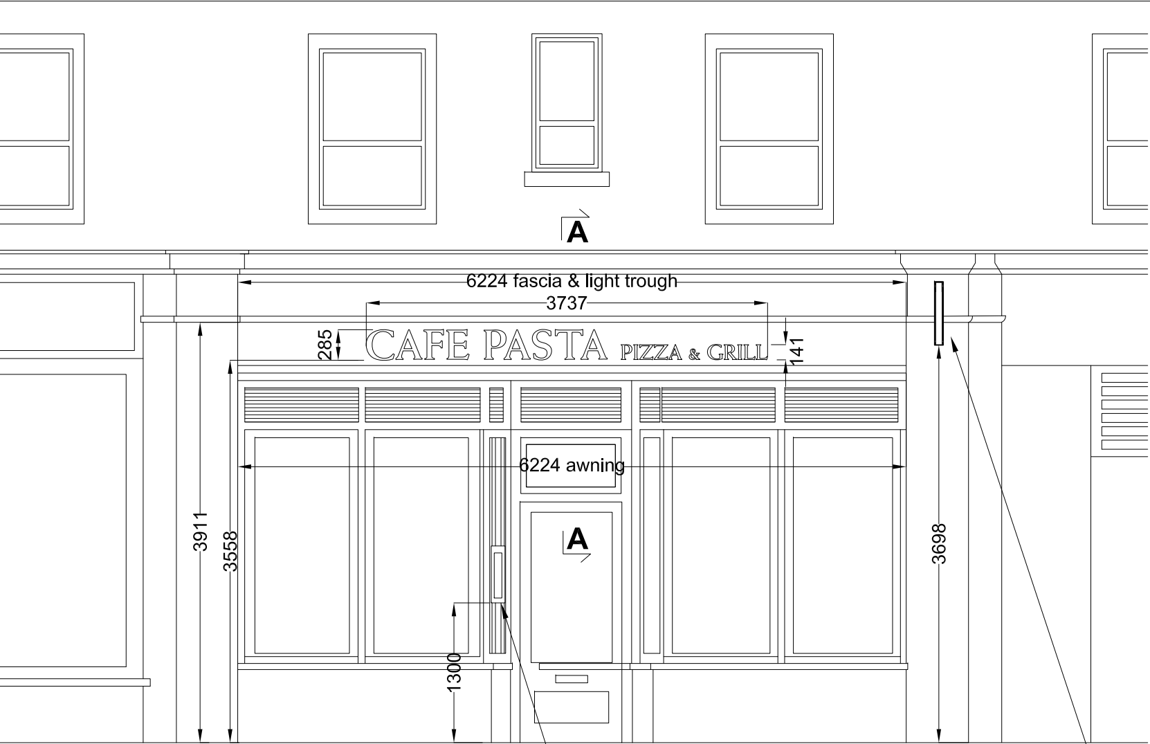
Shaftesbury Avenue Elevation Scale 1:50
