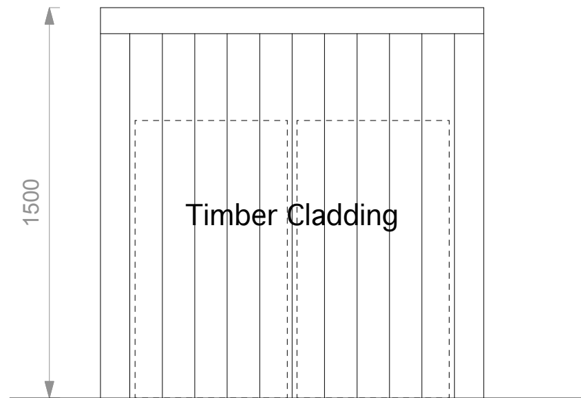
Front Elevation
