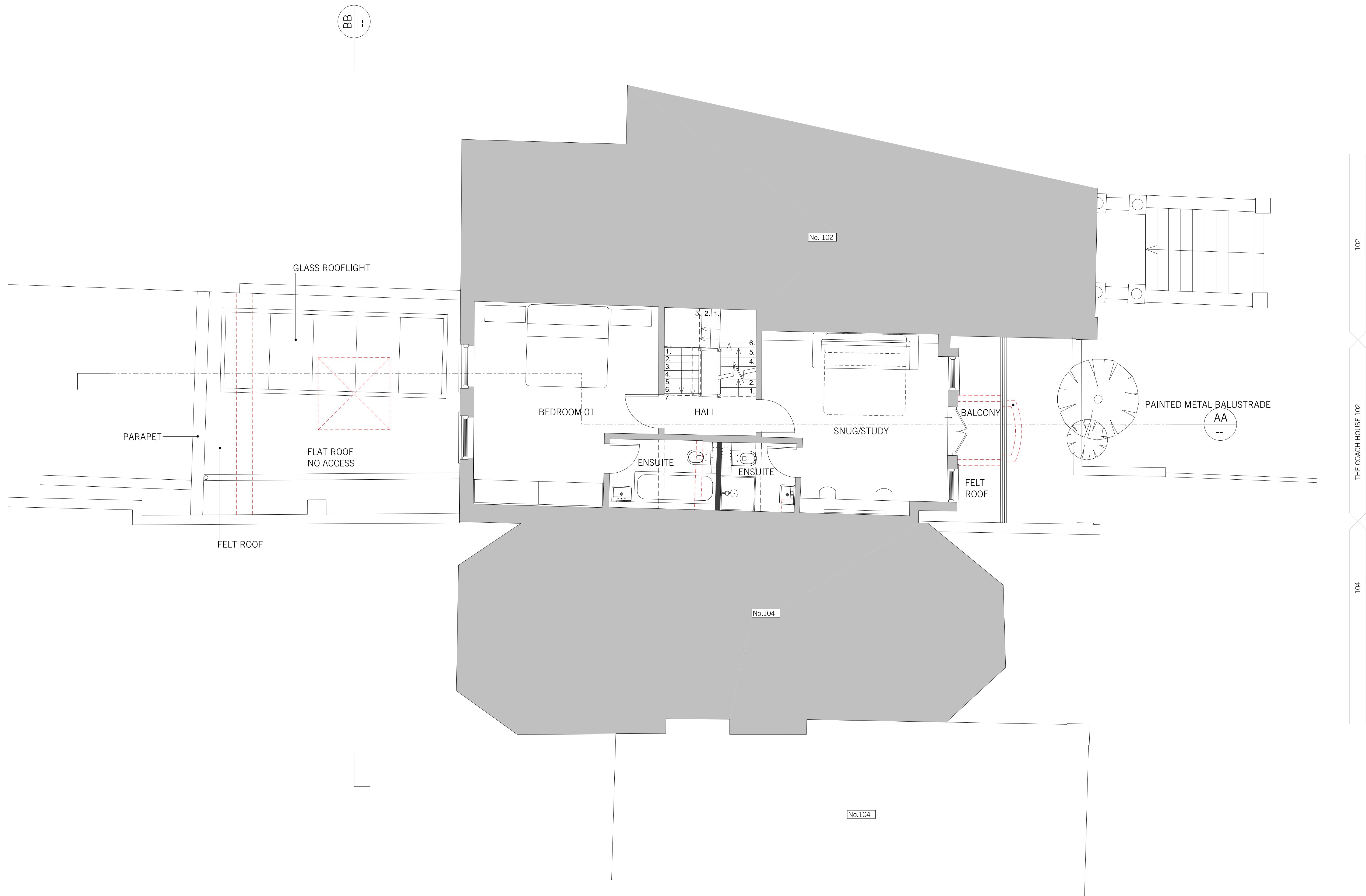
01: PROPOSED FIRST FLOOR PLAN SCALE 1:50
