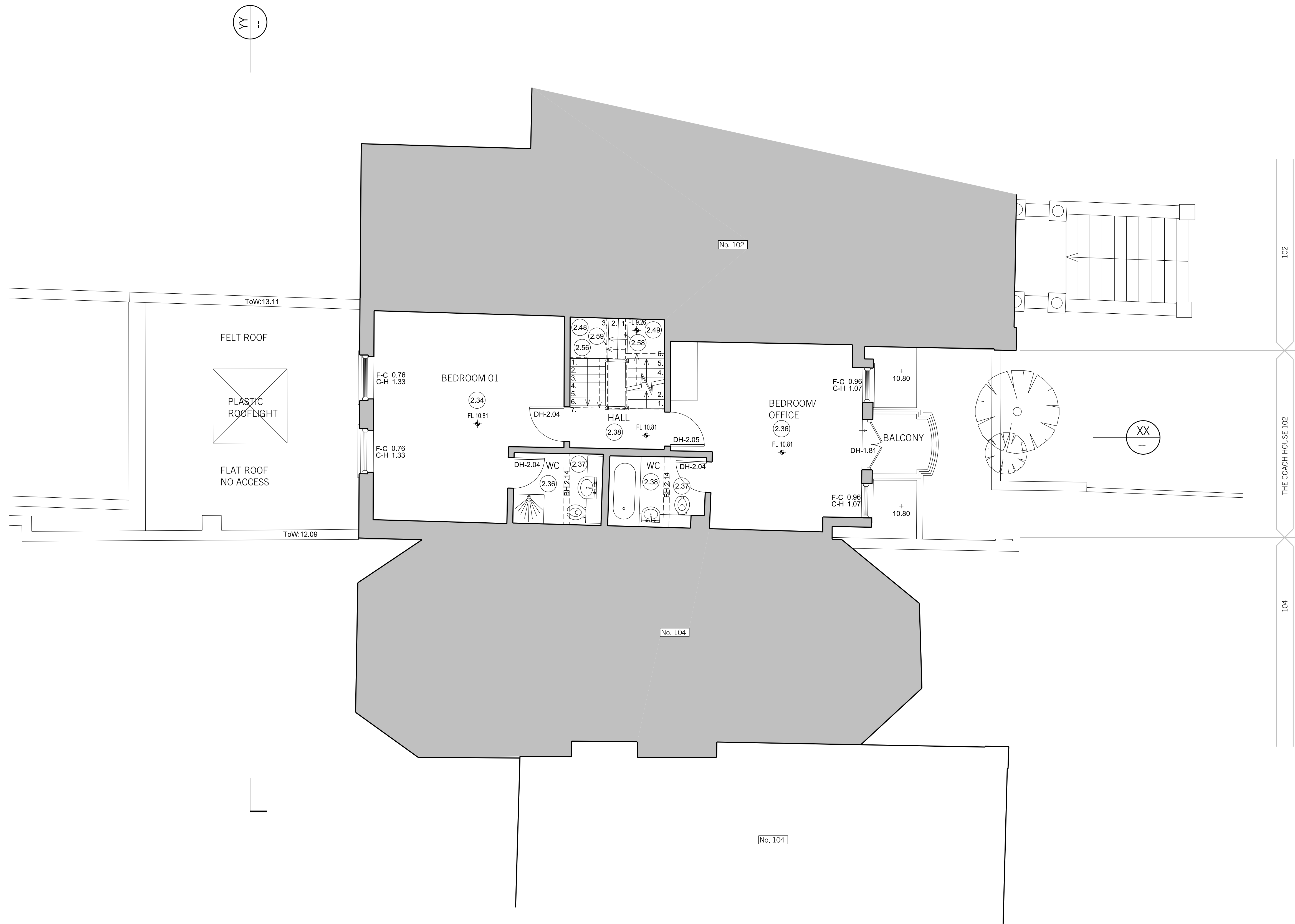
01: EXISTING FIRST FLOOR PLAN SCALE 1:50
