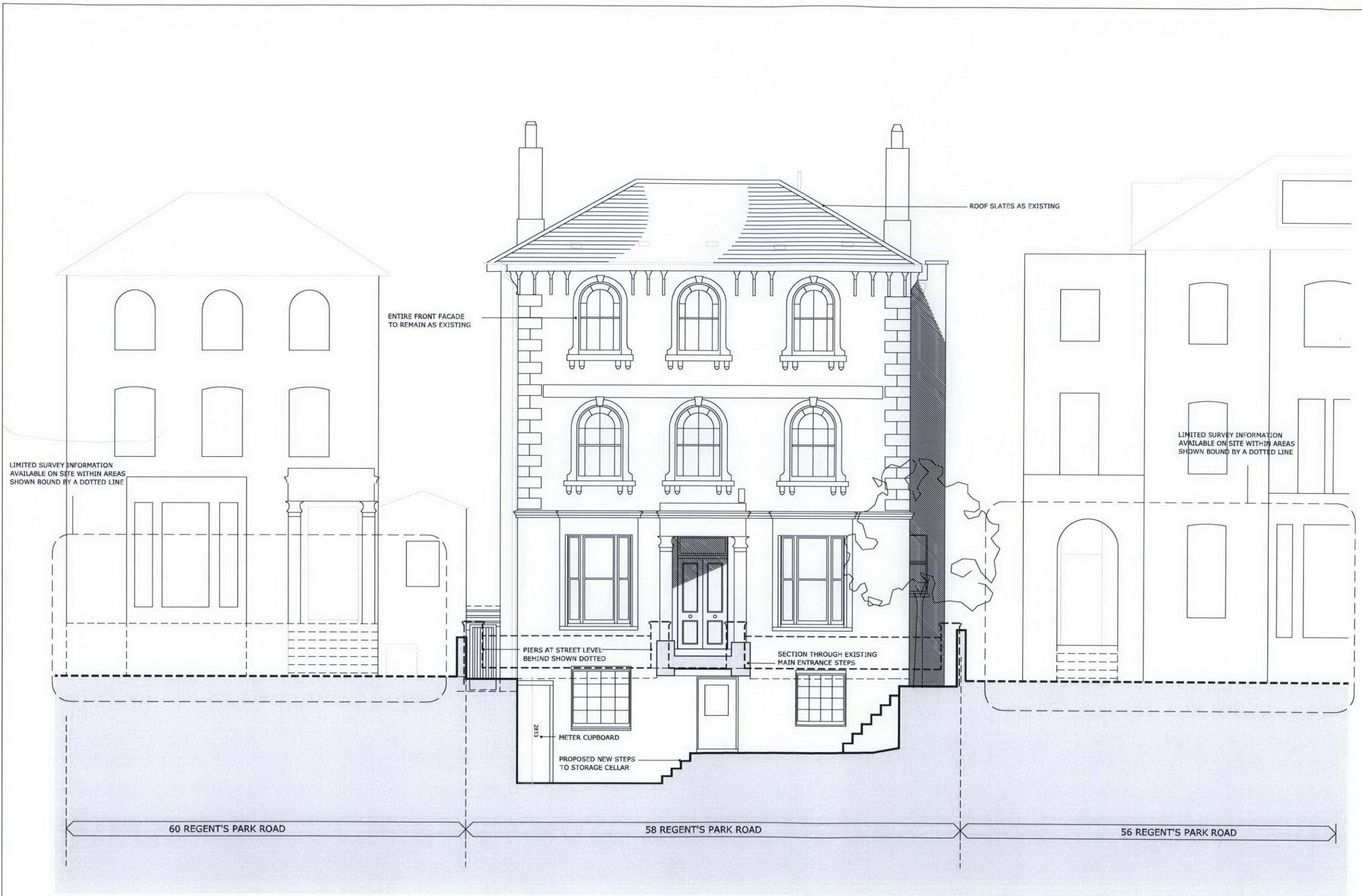
01: SOUTH ELEVATION SCALE 1:50 at A1
